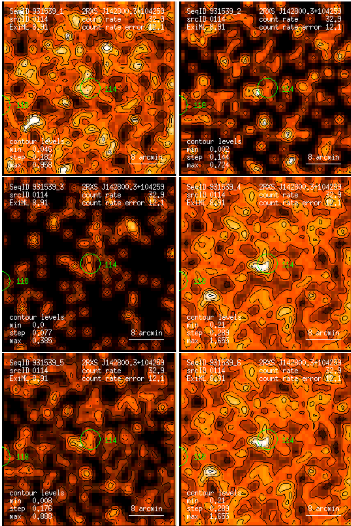
Figure 114: RASS 931539: detection 0114: band rate images, Gaussian filter: (1) PSPC channels 11 – 41, (2) 52 – 90, (3) 91 – 201, (4) 11 – 235, (5) 52 – 201, (6) 11 – 201. Broad band rates in counts/ks. Band rate contour levels in counts/ks/arcmin 2 .
