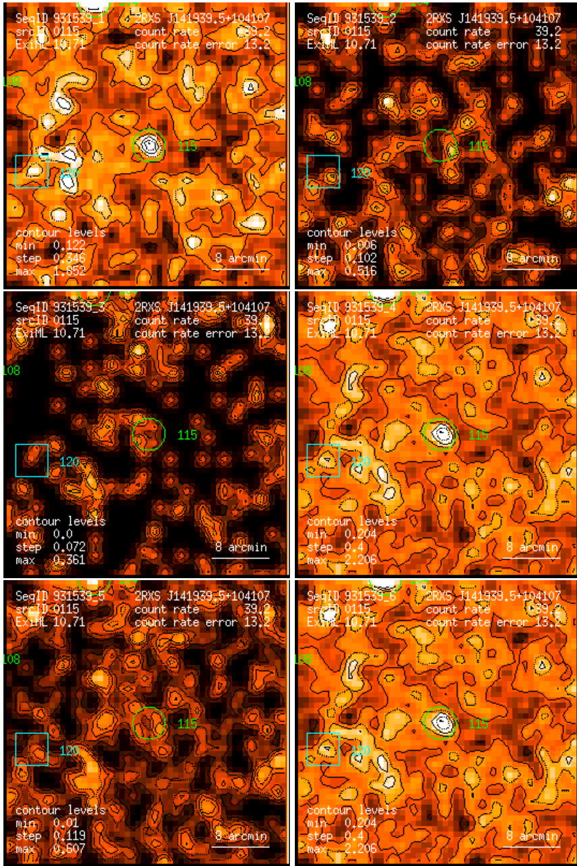
Figure 115: RASS 931539: detection 0115: band rate images, Gaussian filter: (1) PSPC channels 11 – 41, (2) 52 – 90, (3) 91 – 201, (4) 11 – 235, (5) 52 – 201, (6) 11 – 201. Broad band rates in counts/ks. Band rate contour levels in counts/ks/arcmin 2 .
