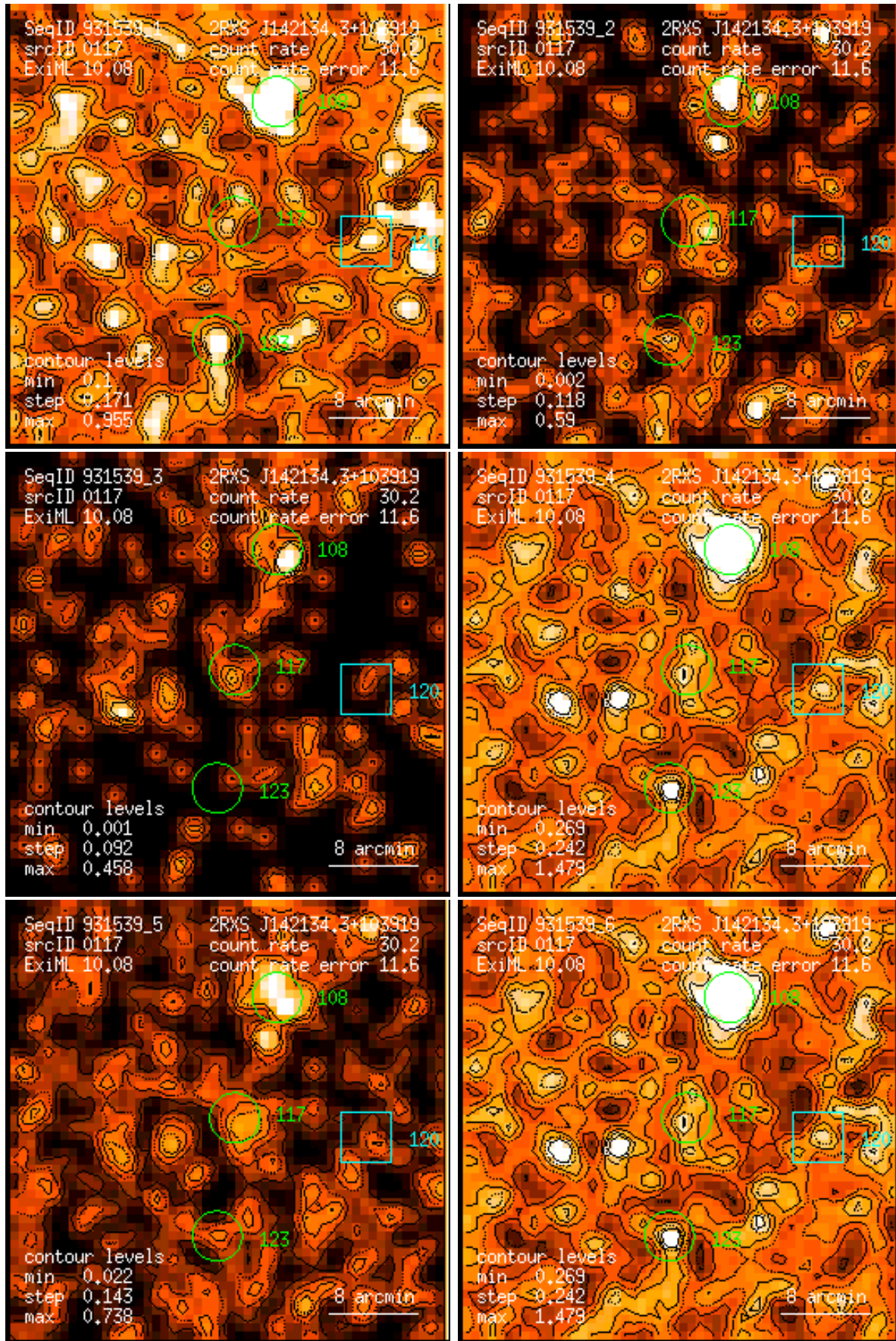
Figure 117: RASS 931539: detection 0117: band rate images, Gaussian filter: (1) PSPC channels 11 – 41, (2) 52 – 90, (3) 91 – 201, (4) 11 – 235, (5) 52 – 201, (6) 11 – 201. Broad band rates in counts/ks. Band rate contour levels in counts/ks/arcmin 2 .
