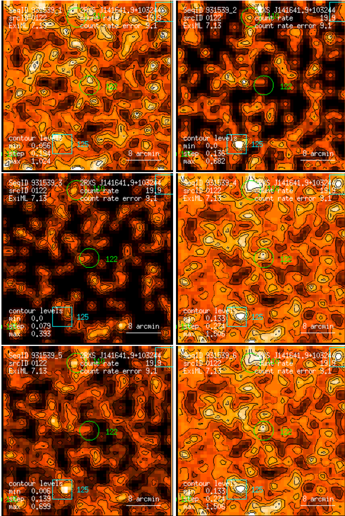
Figure 122: RASS 931539: detection 0122: band rate images, Gaussian filter: (1) PSPC channels 11 – 41, (2) 52 – 90, (3) 91 – 201, (4) 11 – 235, (5) 52 – 201, (6) 11 – 201. Broad band rates in counts/ks. Band rate contour levels in counts/ks/arcmin 2 .
