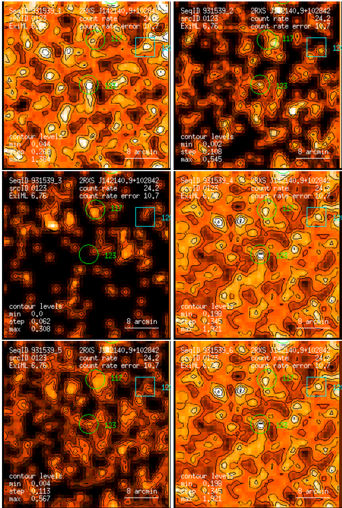
Figure 123: RASS 931539: detection 0123: band rate images, Gaussian filter: (1) PSPC channels 11 – 41, (2) 52 – 90, (3) 91 – 201, (4) 11 – 235, (5) 52 – 201, (6) 11 – 201. Broad band rates in counts/ks. Band rate contour levels in counts/ks/arcmin 2 .
