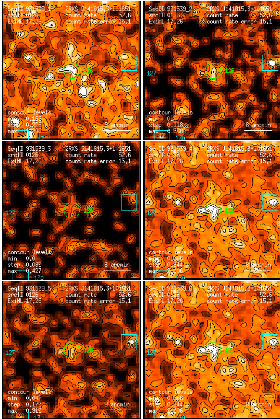
Figure 126: RASS 931539: detection 0126: band rate images, Gaussian filter: (1) PSPC channels 11 – 41, (2) 52 – 90, (3) 91 – 201, (4) 11 – 235, (5) 52 – 201, (6) 11 – 201. Broad band rates in counts/ks. Band rate contour levels in counts/ks/arcmin 2 .
