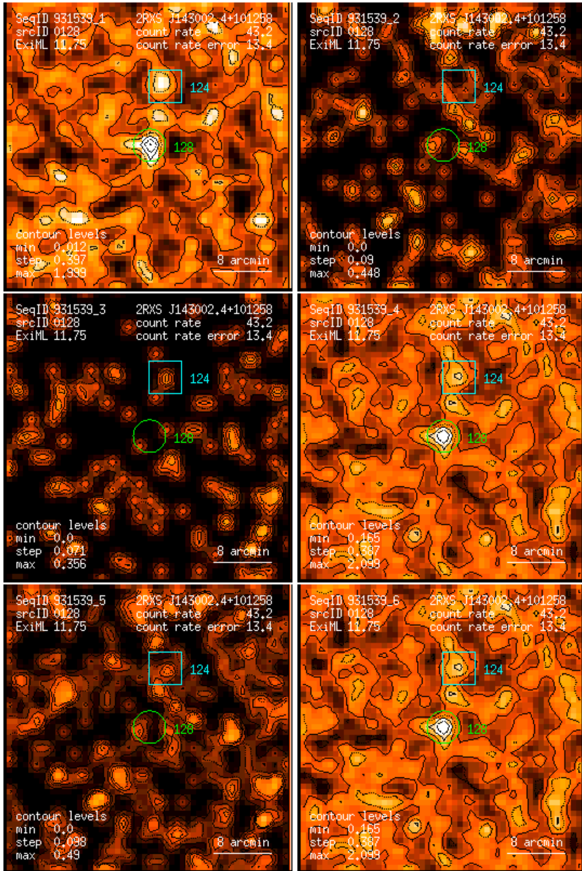
Figure 128: RASS 931539: detection 0128: band rate images, Gaussian filter: (1) PSPC channels 11 – 41, (2) 52 – 90, (3) 91 – 201, (4) 11 – 235, (5) 52 – 201, (6) 11 – 201. Broad band rates in counts/ks. Band rate contour levels in counts/ks/arcmin 2 .
