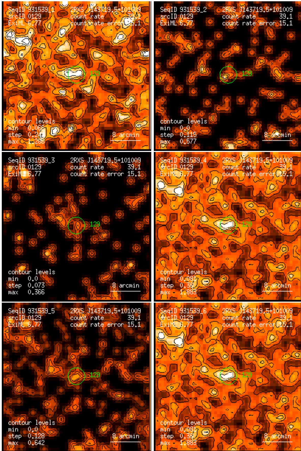
Figure 129: RASS 931539: detection 0129: band rate images, Gaussian filter: (1) PSPC channels 11 – 41, (2) 52 – 90, (3) 91 – 201, (4) 11 – 235, (5) 52 – 201, (6) 11 – 201. Broad band rates in counts/ks. Band rate contour levels in counts/ks/arcmin 2 .
