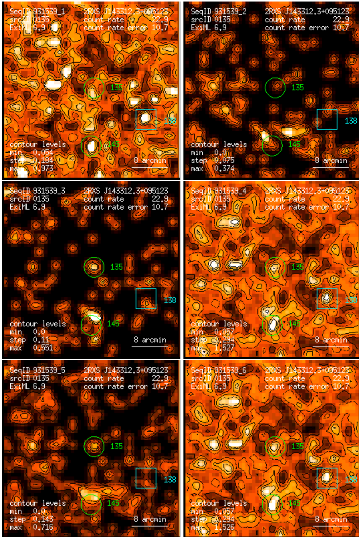
Figure 135: RASS 931539: detection 0135: band rate images, Gaussian filter: (1) PSPC channels 11 – 41, (2) 52 – 90, (3) 91 – 201, (4) 11 – 235, (5) 52 – 201, (6) 11 – 201. Broad band rates in counts/ks. Band rate contour levels in counts/ks/arcmin 2 .
