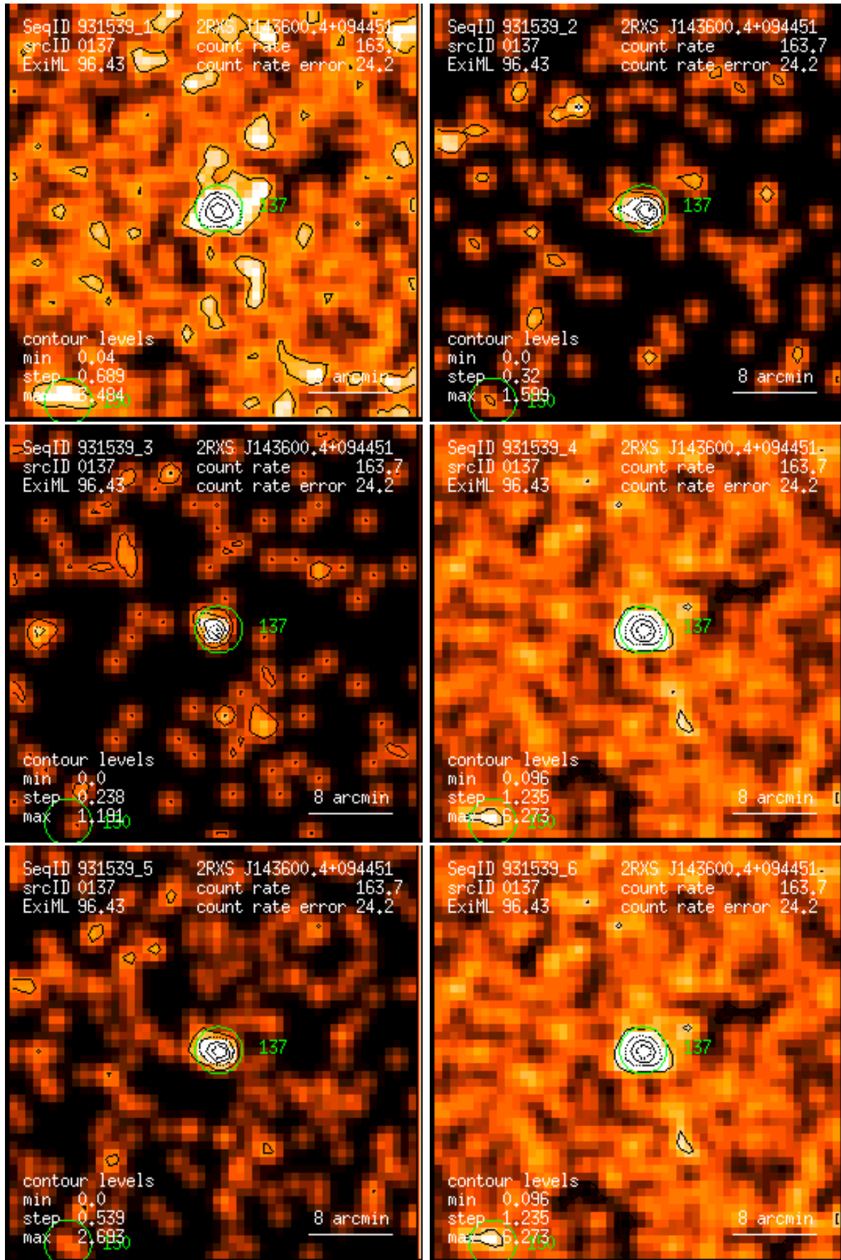
Figure 137: RASS 931539: detection 0137: band rate images, Gaussian filter: (1) PSPC channels 11 – 41, (2) 52 – 90, (3) 91 – 201, (4) 11 – 235, (5) 52 – 201, (6) 11 – 201. Broad band rates in counts/ks. Band rate contour levels in counts/ks/arcmin 2 .
