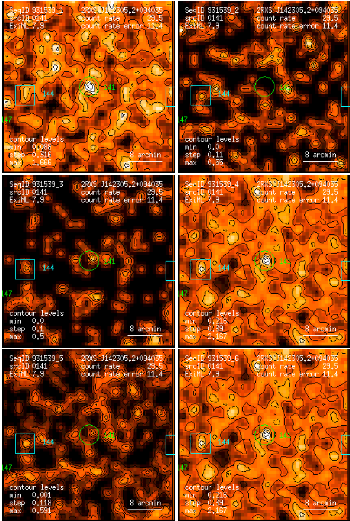
Figure 141: RASS 931539: detection 0141: band rate images, Gaussian filter: (1) PSPC channels 11 – 41, (2) 52 – 90, (3) 91 – 201, (4) 11 – 235, (5) 52 – 201, (6) 11 – 201. Broad band rates in counts/ks. Band rate contour levels in counts/ks/arcmin 2 .
