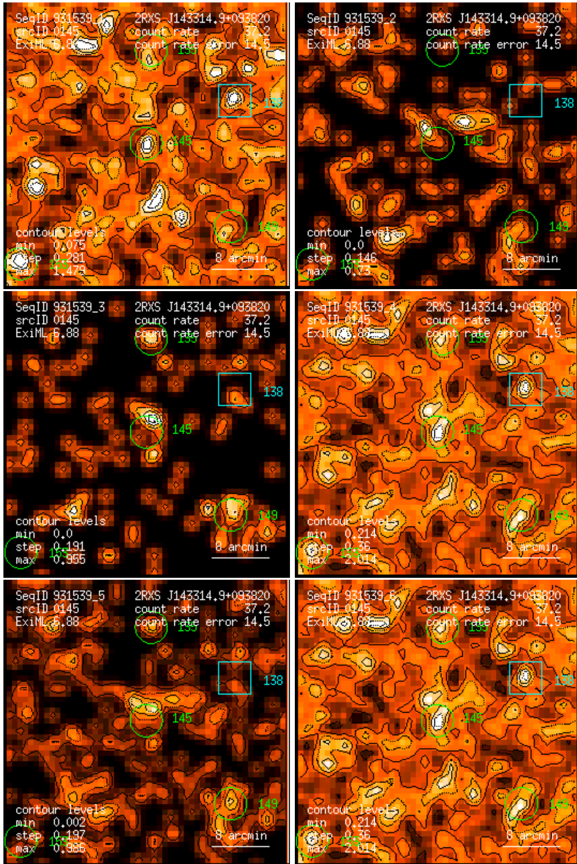
Figure 145: RASS 931539: detection 0145: band rate images, Gaussian filter: (1) PSPC channels 11 – 41, (2) 52 – 90, (3) 91 – 201, (4) 11 – 235, (5) 52 – 201, (6) 11 – 201. Broad band rates in counts/ks. Band rate contour levels in counts/ks/arcmin 2 .
