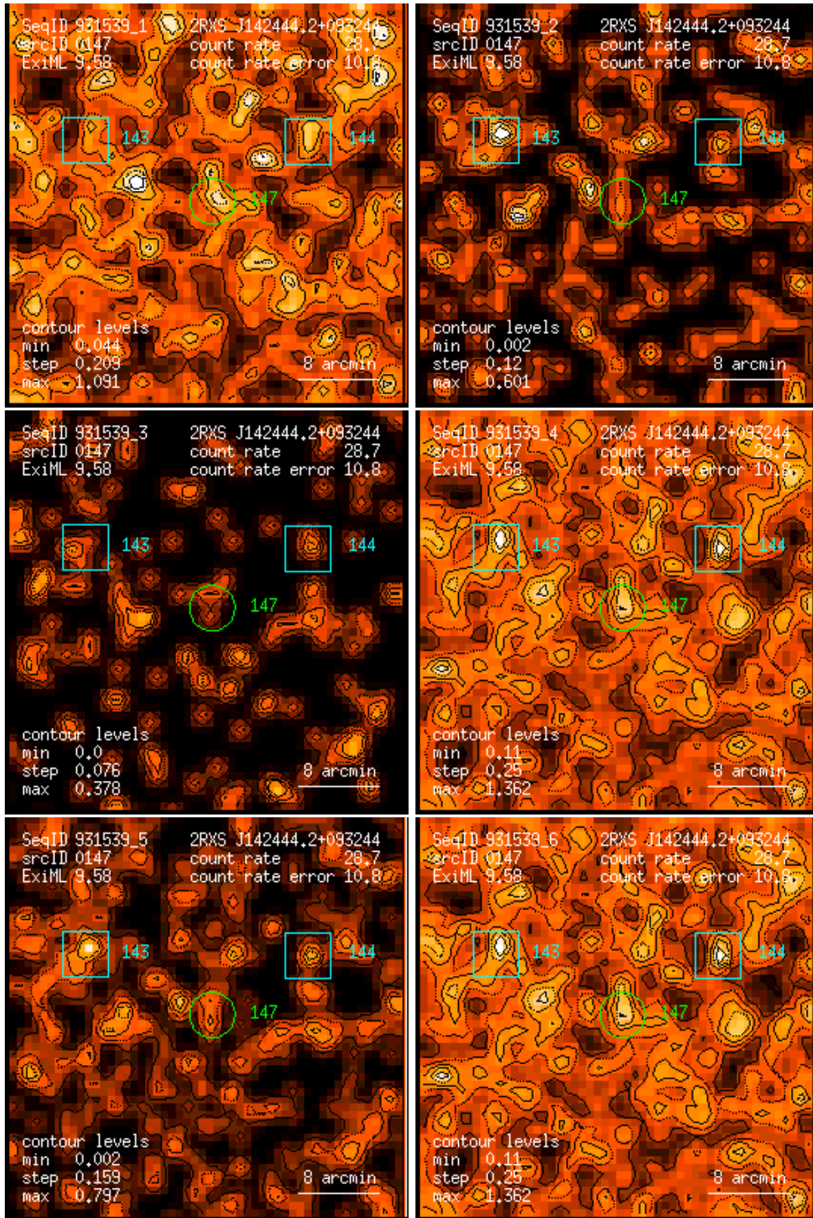
Figure 147: RASS 931539: detection 0147: band rate images, Gaussian filter: (1) PSPC channels 11 – 41, (2) 52 – 90, (3) 91 – 201, (4) 11 – 235, (5) 52 – 201, (6) 11 – 201. Broad band rates in counts/ks. Band rate contour levels in counts/ks/arcmin 2 .
