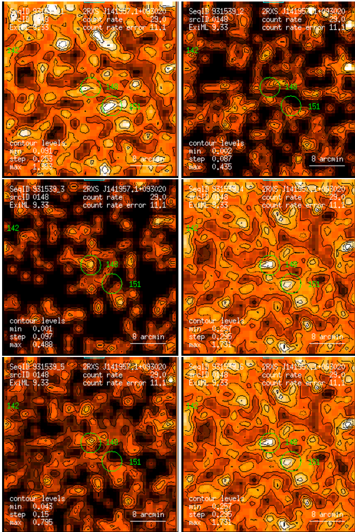
Figure 148: RASS 931539: detection 0148: band rate images, Gaussian filter: (1) PSPC channels 11 – 41, (2) 52 – 90, (3) 91 – 201, (4) 11 – 235, (5) 52 – 201, (6) 11 – 201. Broad band rates in counts/ks. Band rate contour levels in counts/ks/arcmin 2 .
