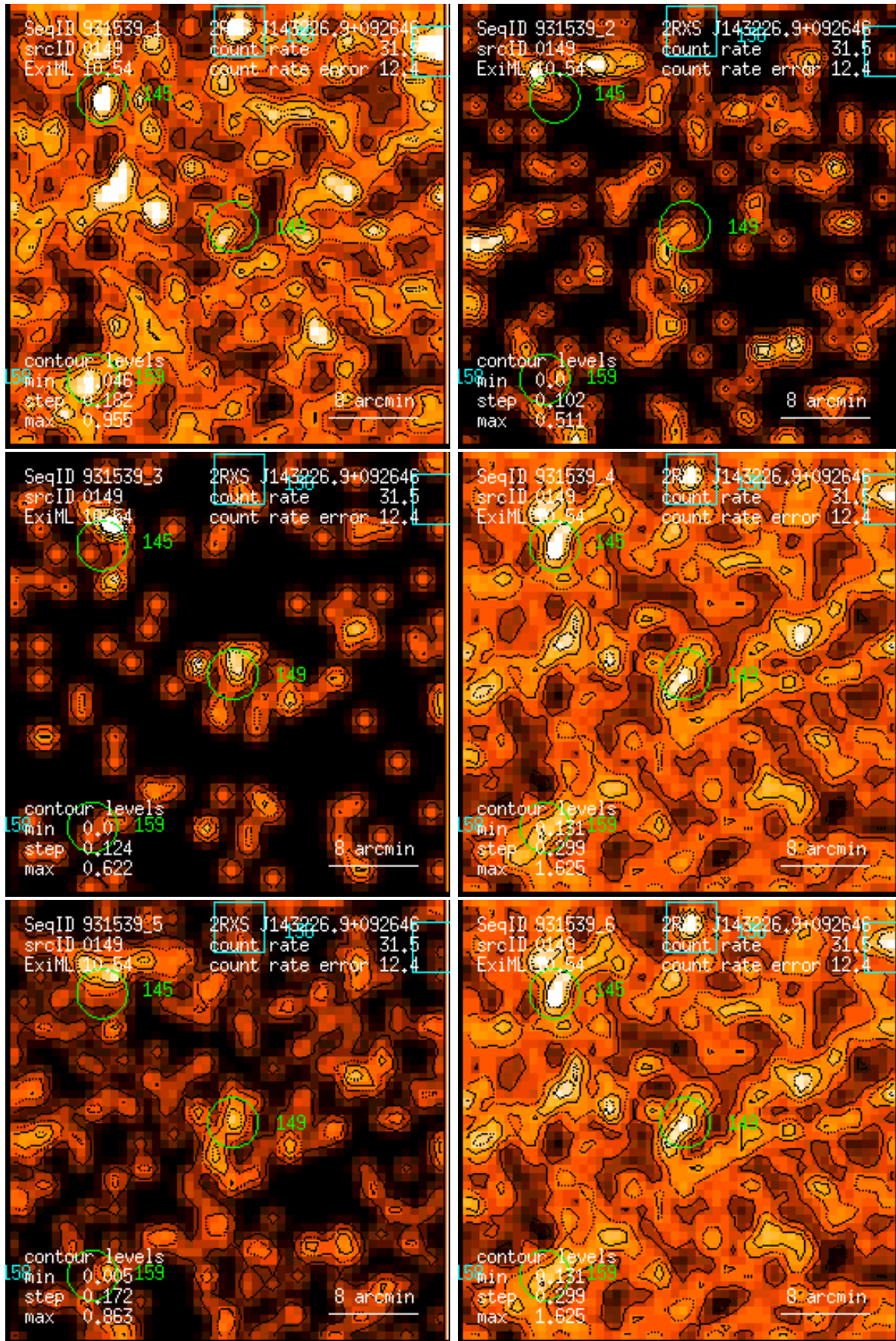
Figure 149: RASS 931539: detection 0149: band rate images, Gaussian filter: (1) PSPC channels 11 – 41, (2) 52 – 90, (3) 91 – 201, (4) 11 – 235, (5) 52 – 201, (6) 11 – 201. Broad band rates in counts/ks. Band rate contour levels in counts/ks/arcmin 2 .
