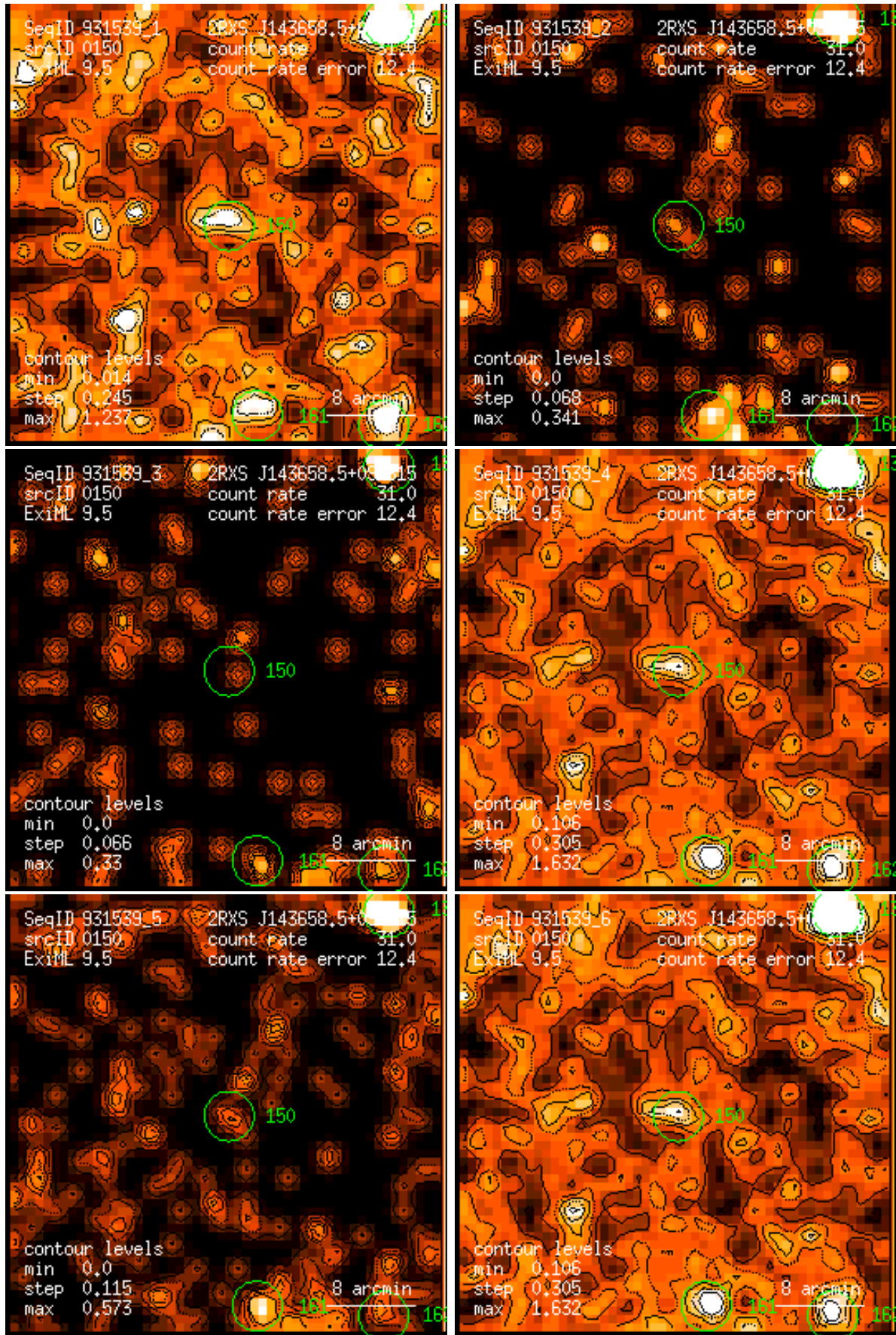
Figure 150: RASS 931539: detection 0150: band rate images, Gaussian filter: (1) PSPPC channels 11 – 41, (2) 52 – 90, (3) 91 – 201, (4) 11 – 235, (5) 52 – 201, (6) 11 – 201. Broad band rates in counts/ks. Band rate contour levels in counts/ks/arcmin 2 .
