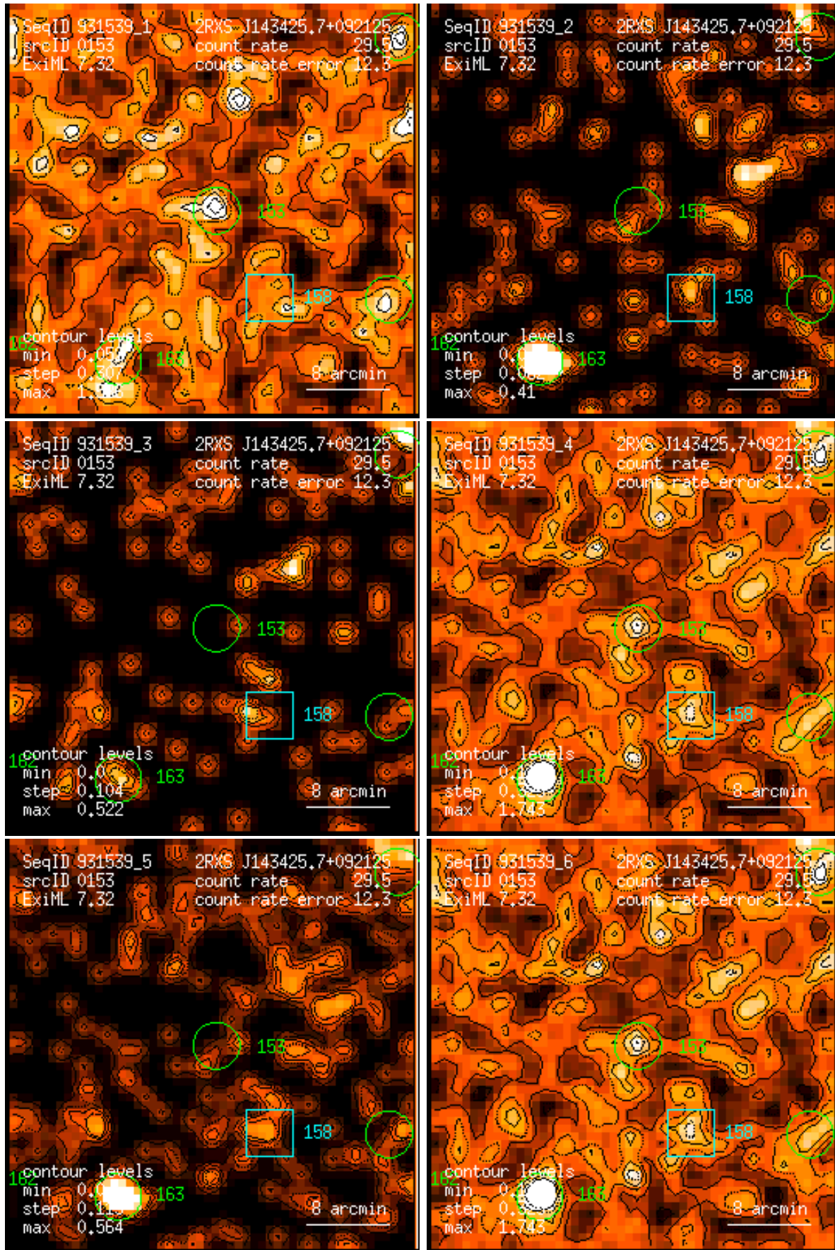
Figure 153: RASS 931539: detection 0153: band rate images, Gaussian filter: (1) PSPC channels 11 – 41, (2) 52 – 90, (3) 91 – 201, (4) 11 – 235, (5) 52 – 201, (6) 11 – 201. Broad band rates in counts/ks. Band rate contour levels in counts/ks/arcmin 2 .
