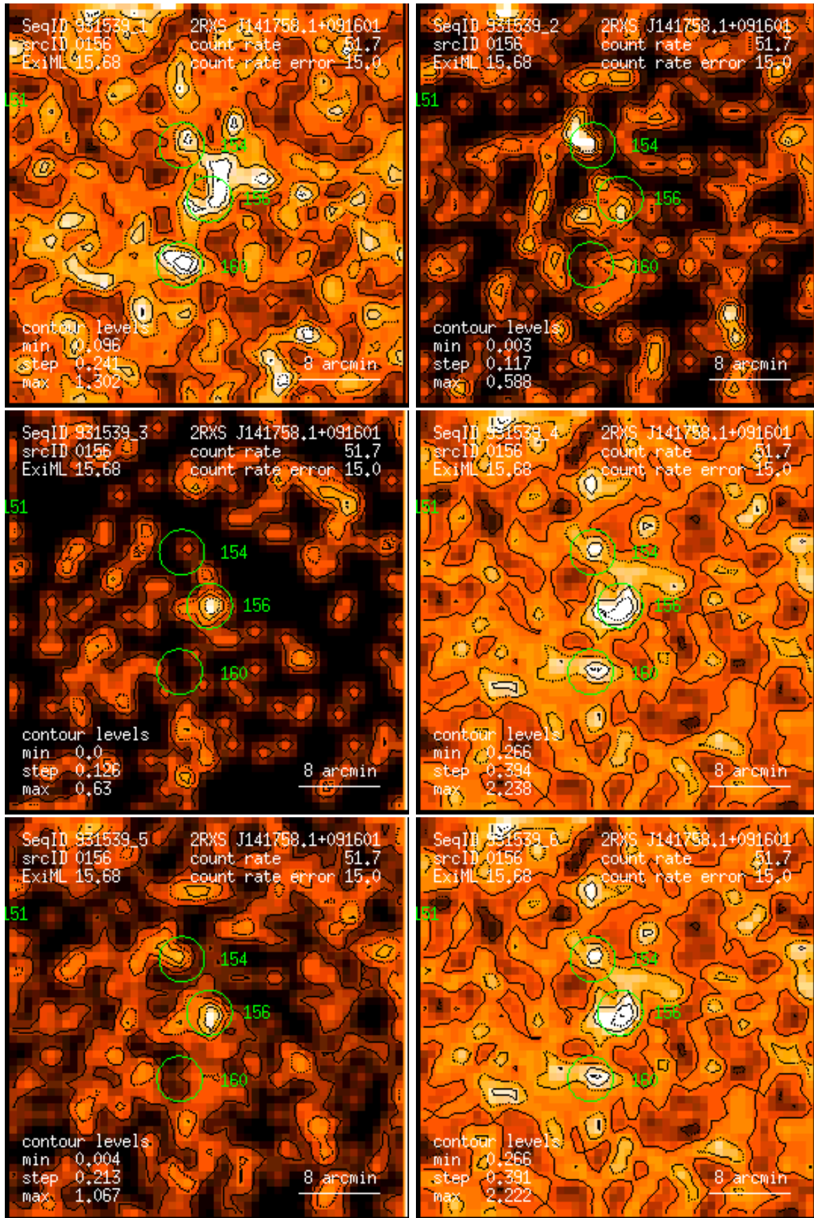
Figure 156: RASS 931539: detection 0156: band rate images, Gaussian filter: (1) PSPC channels 11 – 41, (2) 52 – 90, (3) 91 – 201, (4) 11 – 235, (5) 52 – 201, (6) 11 – 201. Broad band rates in counts/ks. Band rate contour levels in counts/ks/arcmin 2 .
