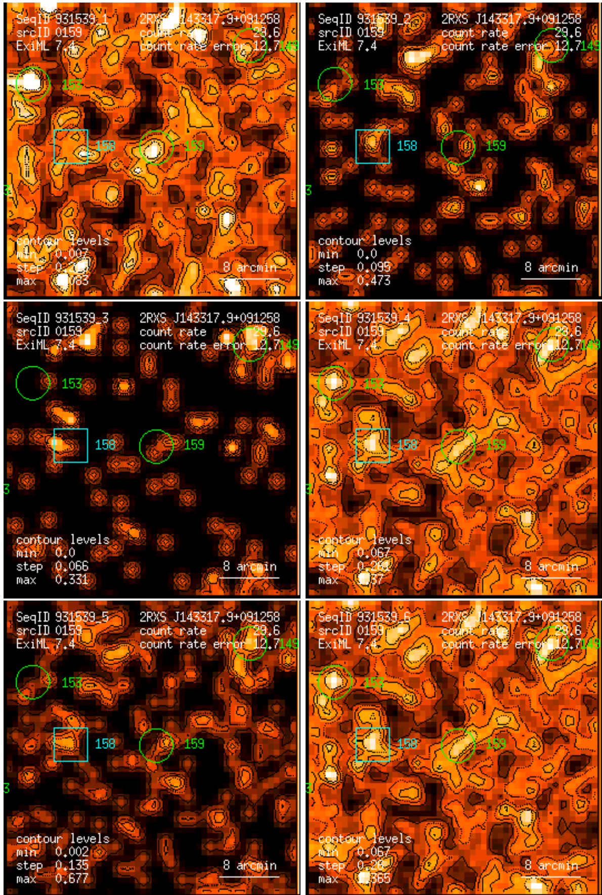
Figure 159: RASS 931539: detection 0159: band rate images, Gaussian filter: (1) PSPC channels 11 – 41, (2) 52 – 90, (3) 91 – 201, (4) 11 – 235, (5) 52 – 201, (6) 11 – 201. Broad band rates in counts/ks. Band rate contour levels in counts/ks/arcmin 2 .
