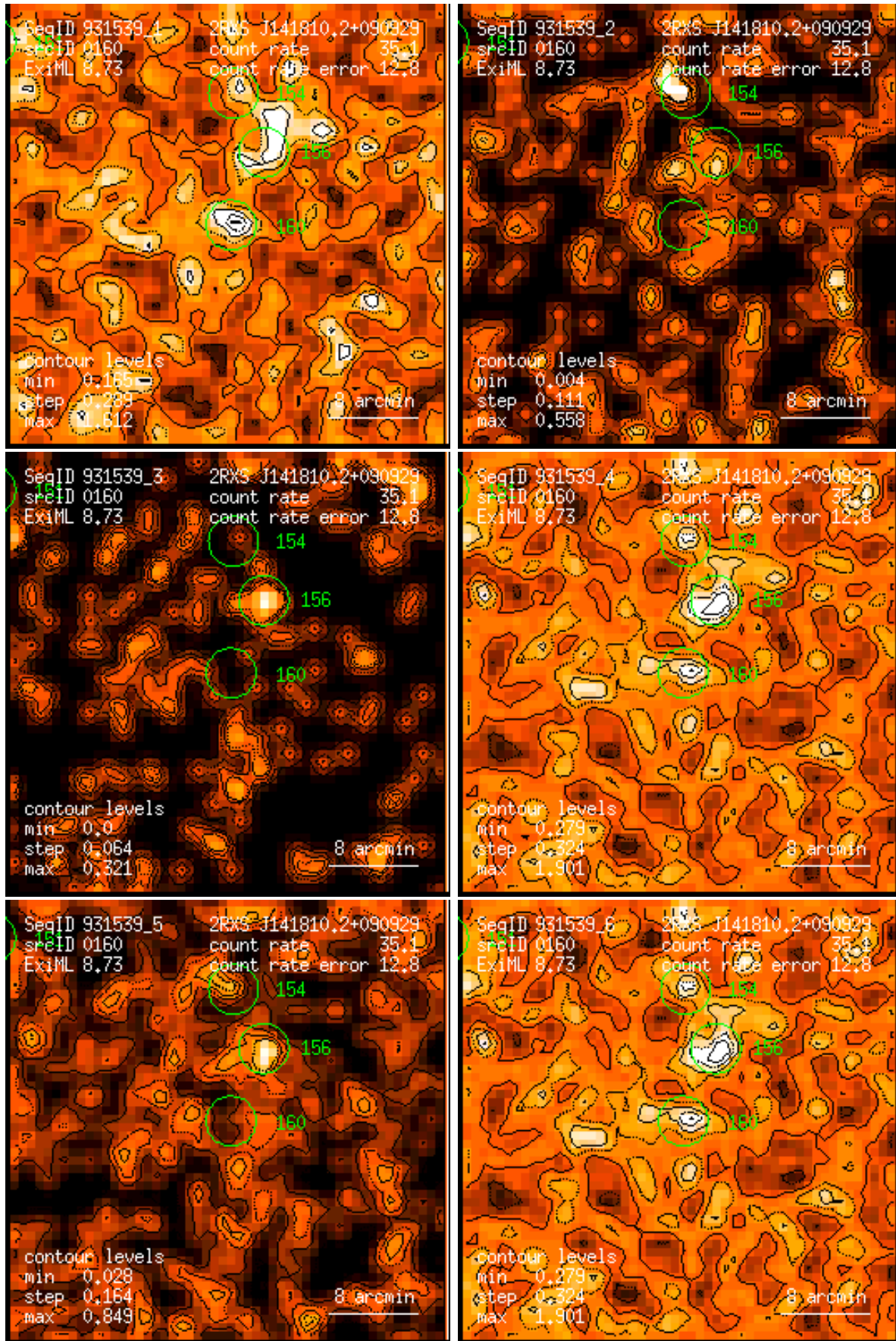
Figure 160: RASS 931539: detection 0160: band rate images, Gaussian filter: (1) PSPC channels 11 – 41, (2) 52 – 90, (3) 91 – 201, (4) 11 – 235, (5) 52 – 201, (6) 11 – 201. Broad band rates in counts/ks. Band rate contour levels in counts/ks/arcmin 2 .
