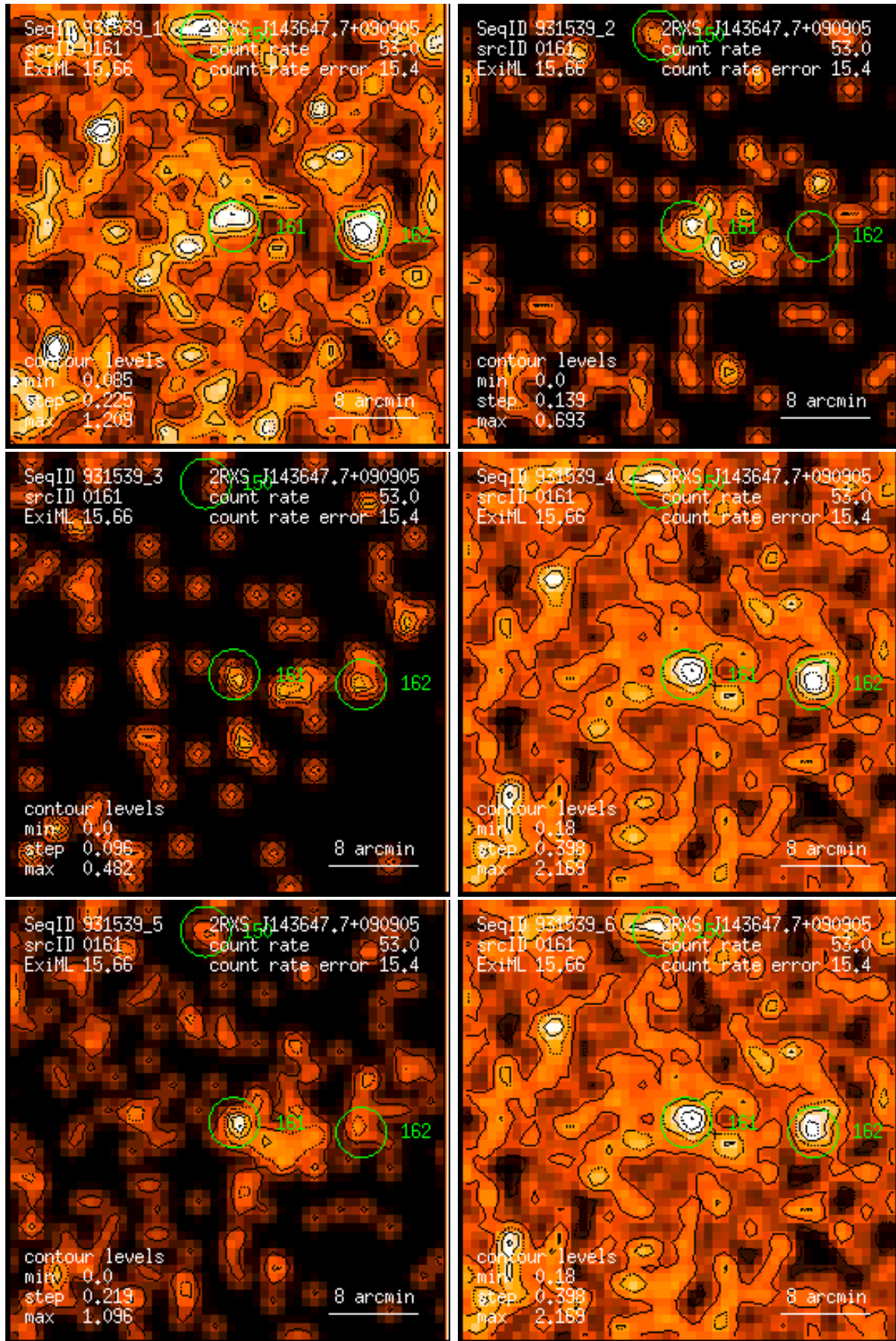
Figure 161: RASS 931539: detection 0161: band rate images, Gaussian filter: (1) PSPC channels 11 – 41, (2) 52 – 90, (3) 91 – 201, (4) 11 – 235, (5) 52 – 201, (6) 11 – 201. Broad band rates in counts/ks. Band rate contour levels in counts/ks/arcmin 2 .
