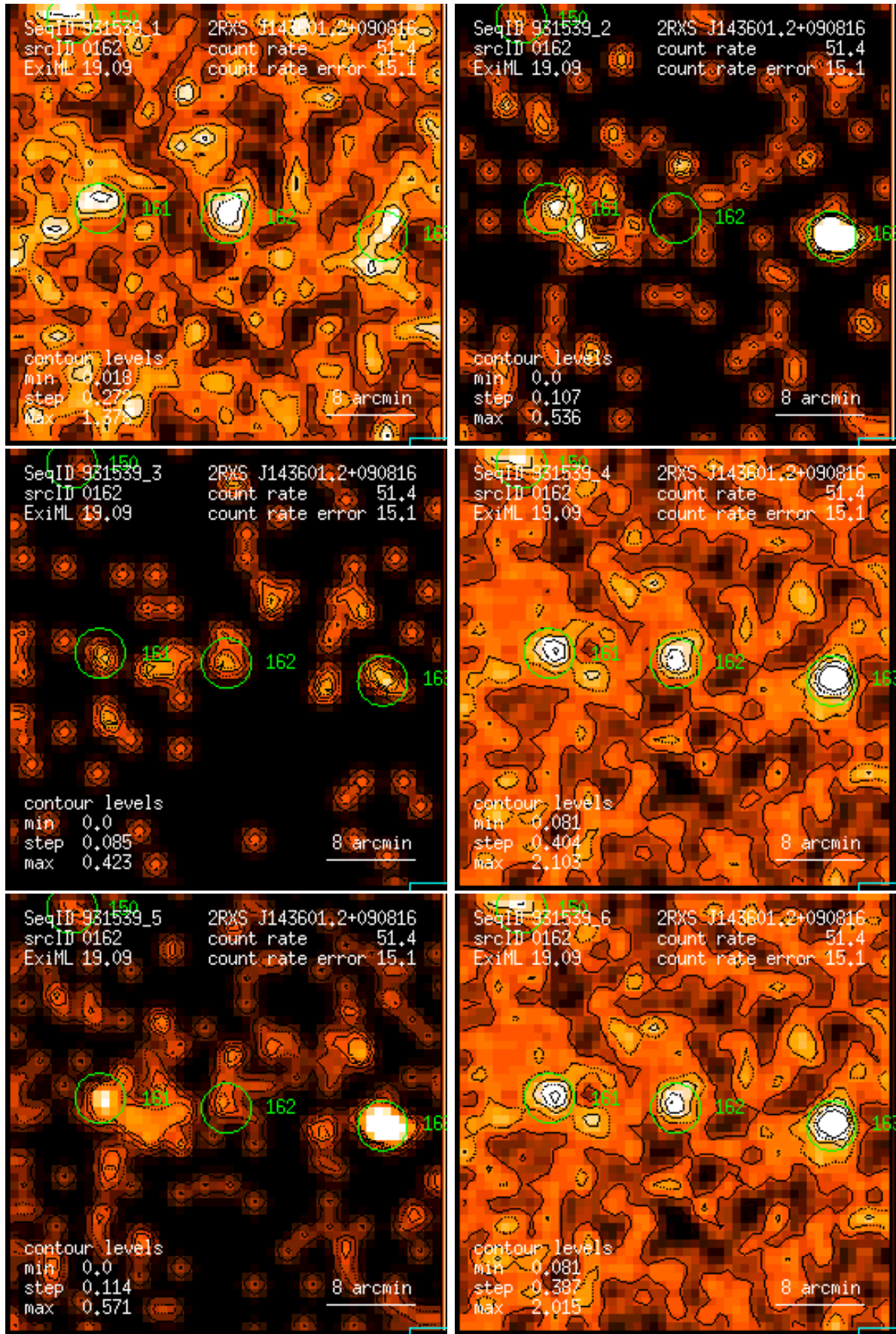
Figure 162: RASS 931539: detection 0162: band rate images, Gaussian filter: (1) PSPC channels 11 – 41, (2) 52 – 90, (3) 91 – 201, (4) 11 – 235, (5) 52 – 201, (6) 11 – 201. Broad band rates in counts/ks. Band rate contour levels in counts/ks/arcmin 2 .
