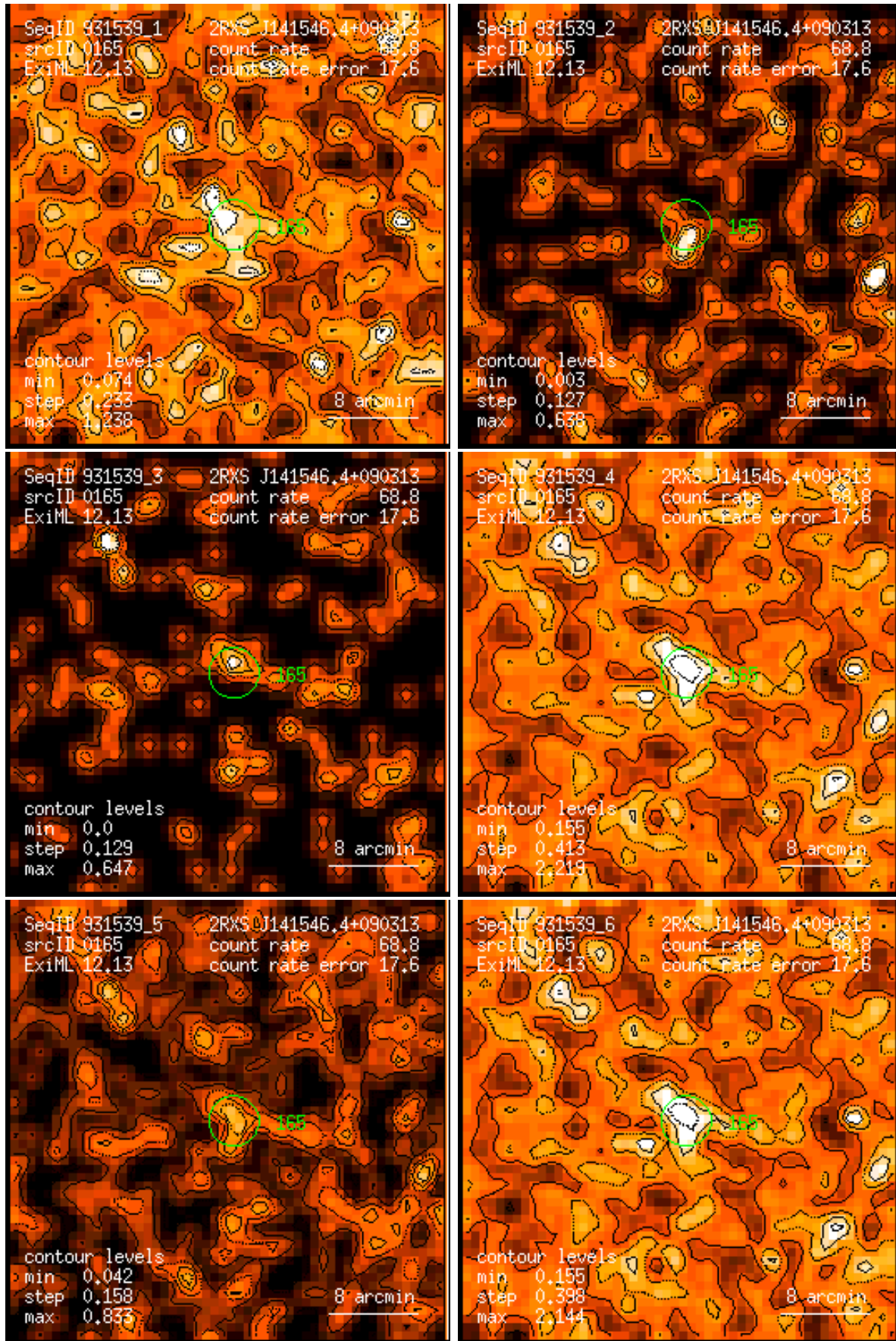
Figure 165: RASS 931539: detection 0165: band rate images, Gaussian filter: (1) PSPC channels 11 – 41, (2) 52 – 90, (3) 91 – 201, (4) 11 – 235, (5) 52 – 201, (6) 11 – 201. Broad band rates in counts/ks. Band rate contour levels in counts/ks/arcmin 2 .
