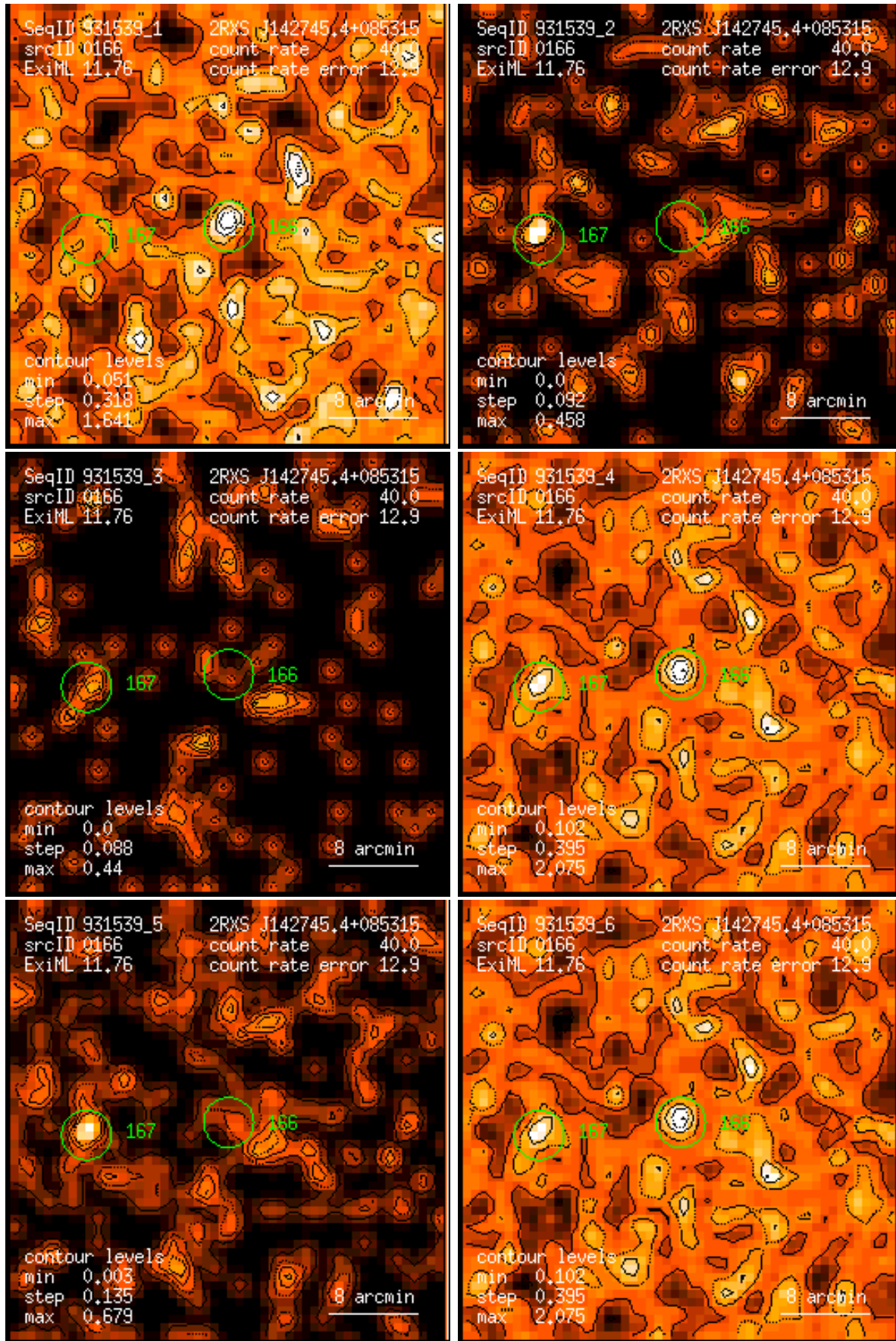
Figure 166: RASS 931539: detection 0166: band rate images, Gaussian filter: (1) PSPC channels 11 – 41, (2) 52 – 90, (3) 91 – 201, (4) 11 – 235, (5) 52 – 201, (6) 11 – 201. Broad band rates in counts/ks. Band rate contour levels in counts/ks/arcmin 2 .
