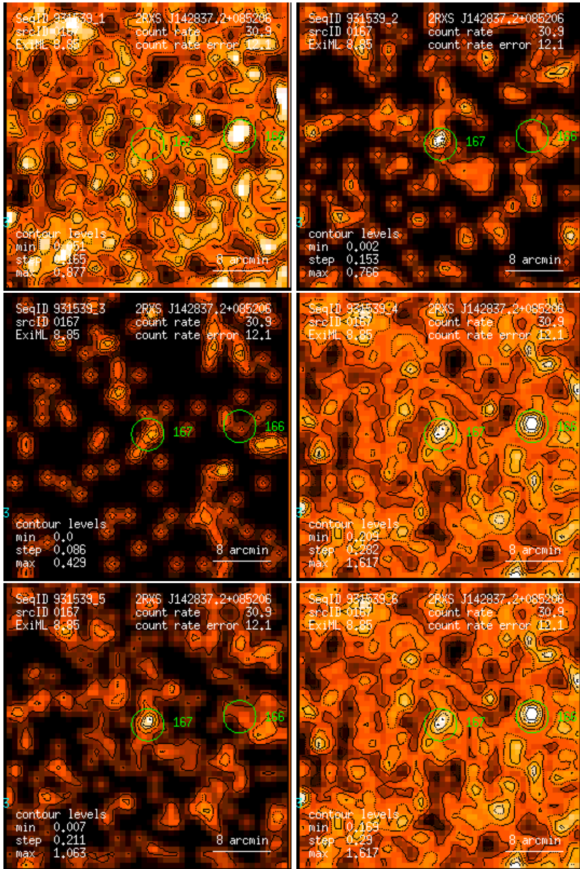
Figure 167: RASS 931539: detection 0167: band rate images, Gaussian filter: (1) PSPC channels 11 – 41, (2) 52 – 90, (3) 91 – 201, (4) 11 – 235, (5) 52 – 201, (6) 11 – 201. Broad band rates in counts/ks. Band rate contour levels in counts/ks/arcmin 2 .
