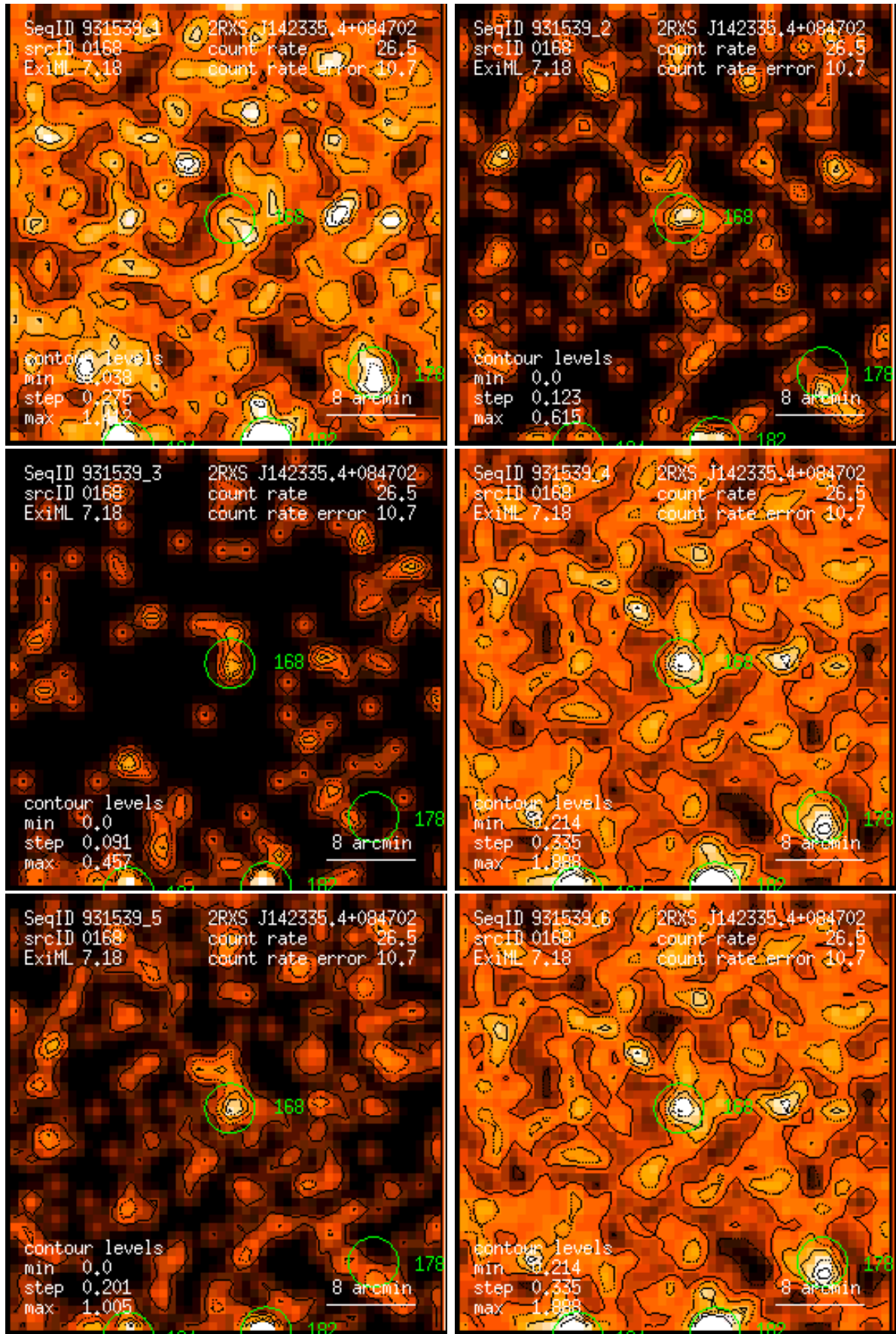
Figure 168: RASS 931539: detection 0168: band rate images, Gaussian filter: (1) PSPC channels 11 – 41, (2) 52 – 90, (3) 91 – 201, (4) 11 – 235, (5) 52 – 201, (6) 11 – 201. Broad band rates in counts/ks. Band rate contour levels in counts/ks/arcmin 2 .
