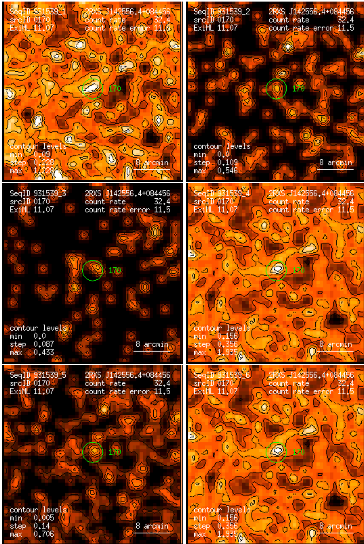
Figure 170: RASS 931539: detection 0170: band rate images, Gaussian filter: (1) PSPC channels 11 – 41, (2) 52 – 90, (3) 91 – 201, (4) 11 – 235, (5) 52 – 201, (6) 11 – 201. Broad band rates in counts/ks. Band rate contour levels in counts/ks/arcmin 2 .
