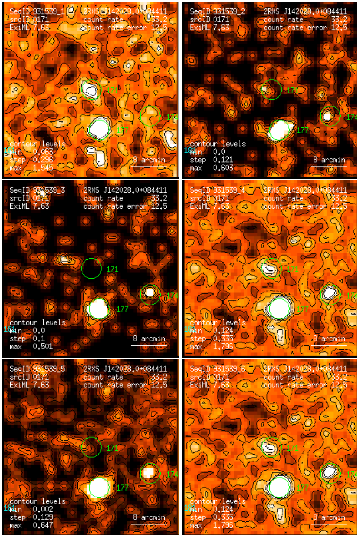
Figure 171: RASS 931539: detection 0171: band rate images, Gaussian filter: (1) PSPC channels 11 – 41, (2) 52 – 90, (3) 91 – 201, (4) 11 – 235, (5) 52 – 201, (6) 11 – 201. Broad band rates in counts/ks. Band rate contour levels in counts/ks/arcmin 2 .
