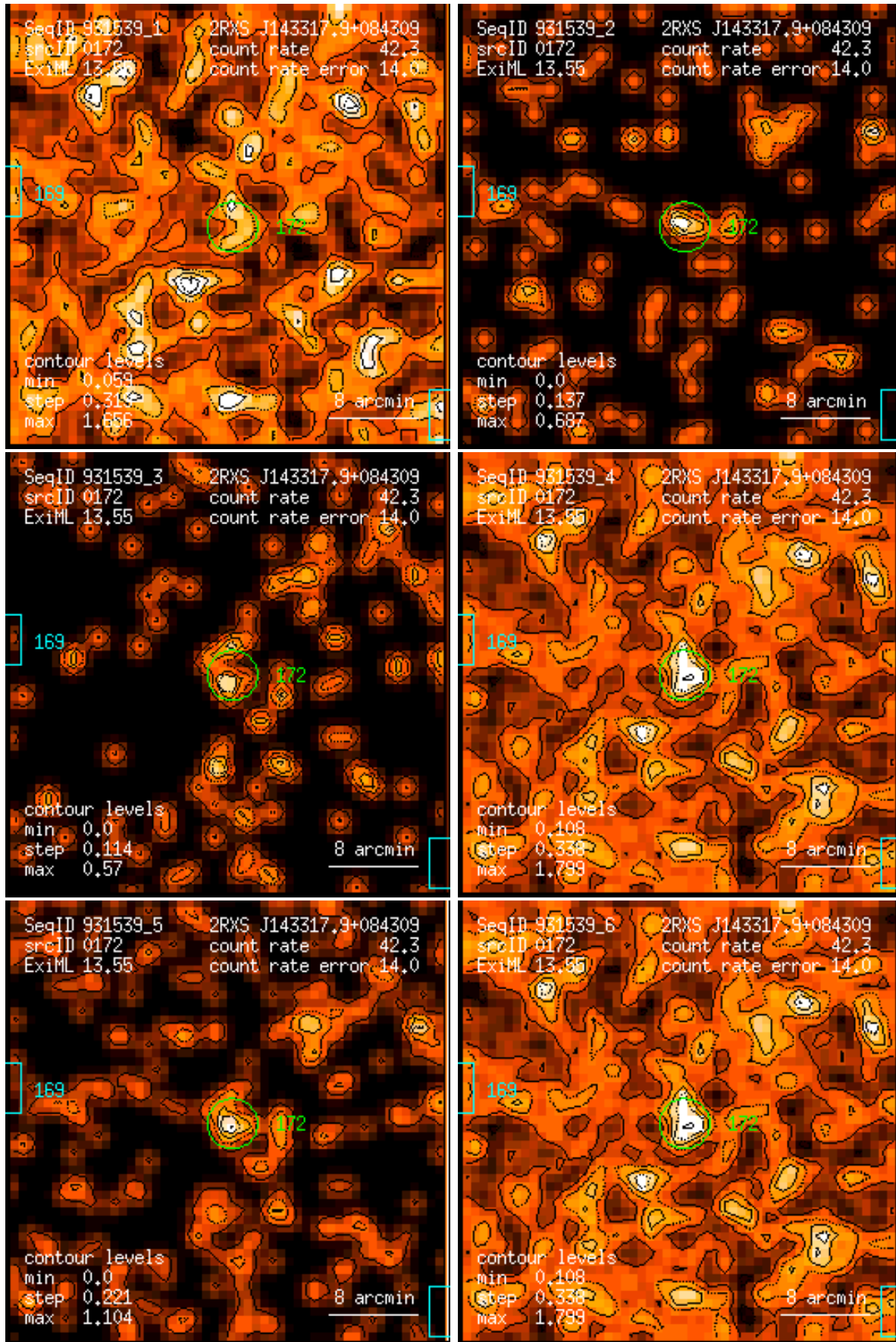
Figure 172: RASS 931539: detection 0172: band rate images, Gaussian filter: (1) PSPC channels 11 – 41, (2) 52 – 90, (3) 91 – 201, (4) 11 – 235, (5) 52 – 201, (6) 11 – 201. Broad band rates in counts/ks. Band rate contour levels in counts/ks/arcmin 2 .
