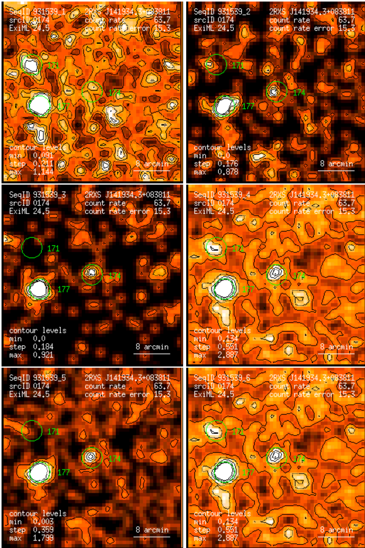
Figure 174: RASS 931539: detection 0174: band rate images, Gaussian filter: (1) PSPC channels 11 – 41, (2) 52 – 90, (3) 91 – 201, (4) 11 – 235, (5) 52 – 201, (6) 11 – 201. Broad band rates in counts/ks. Band rate contour levels in counts/ks/arcmin 2 .
