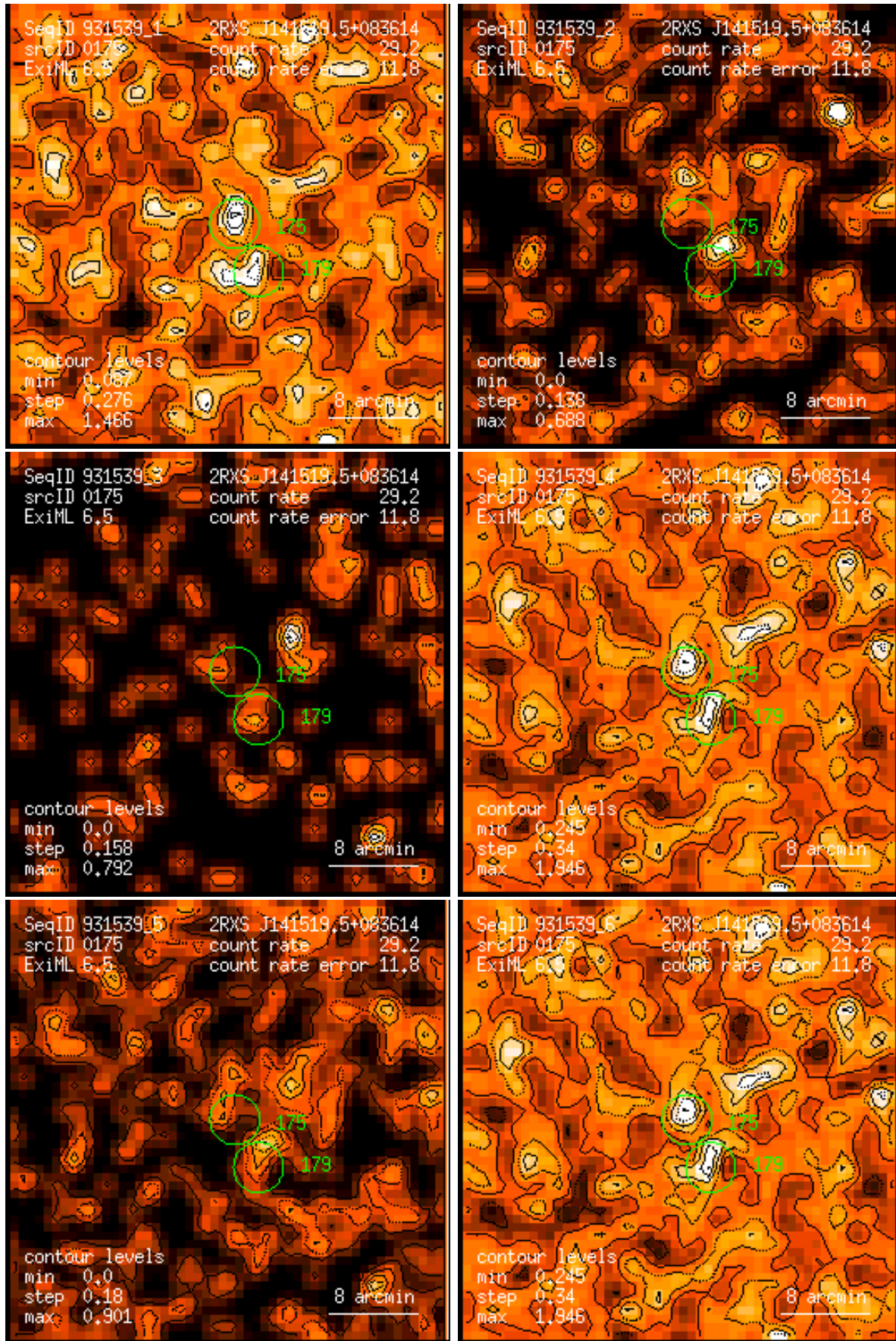
Figure 175: RASS 931539: detection 0175: band rate images, Gaussian filter: (1) PSPC channels 11 – 41, (2) 52 – 90, (3) 91 – 201, (4) 11 – 235, (5) 52 – 201, (6) 11 – 201. Broad band rates in counts/ks. Band rate contour levels in counts/ks/arcmin 2 .
