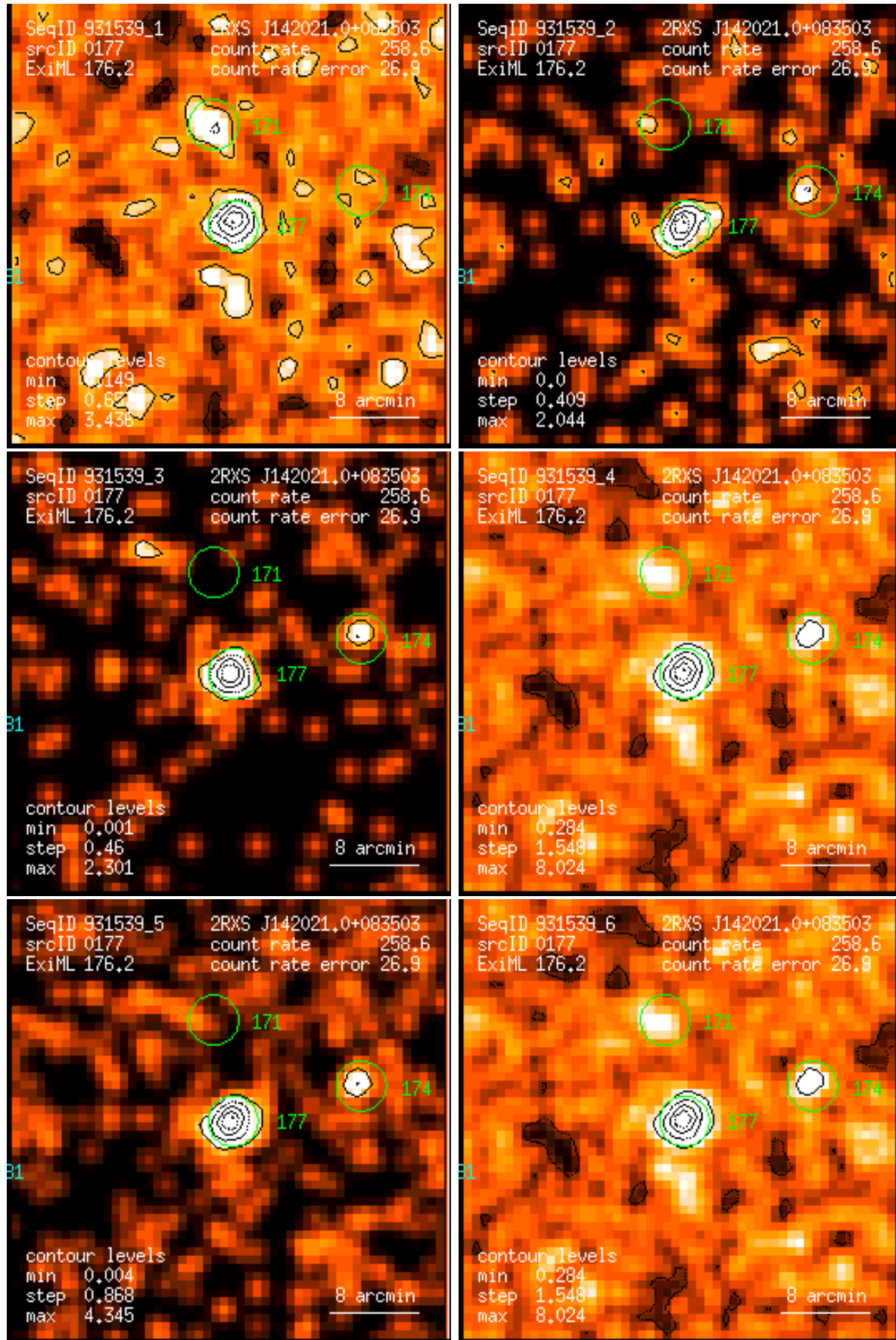
Figure 177: RASS 931539: detection 0177: band rate images, Gaussian filter: (1) PSPC channels 11 – 41, (2) 52 – 90, (3) 91 – 201, (4) 11 – 235, (5) 52 – 201, (6) 11 – 201. Broad band rates in counts/ks. Band rate contour levels in counts/ks/arcmin 2 .
