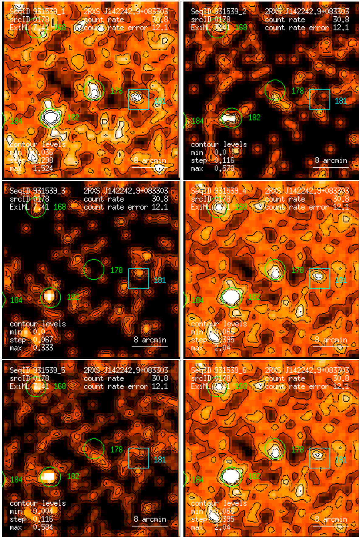
Figure 178: RASS 931539: detection 0178: band rate images, Gaussian filter: (1) PSPC channels 11 – 41, (2) 52 – 90, (3) 91 – 201, (4) 11 – 235, (5) 52 – 201, (6) 11 – 201. Broad band rates in counts/ks. Band rate contour levels in counts/ks/arcmin 2 .
