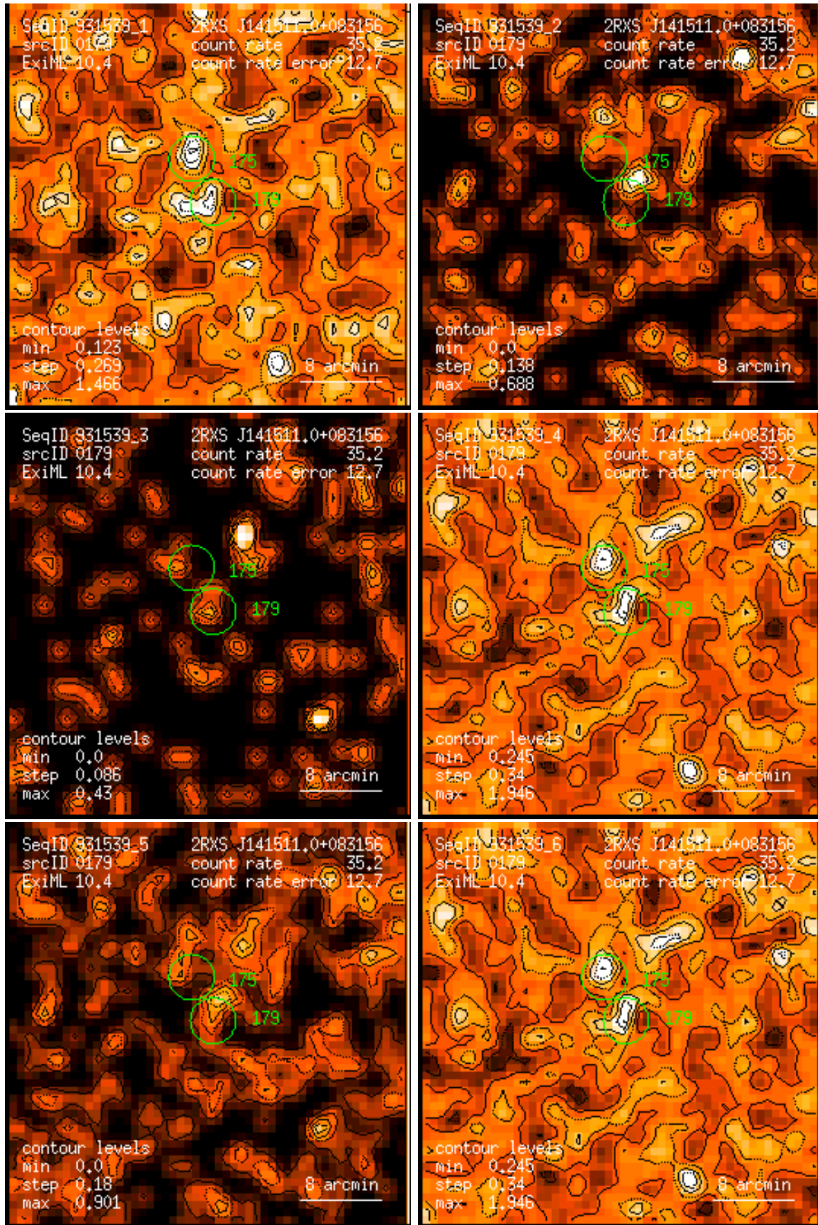
Figure 179: RASS 931539: detection 0179: band rate images, Gaussian filter: (1) PSPC channels 11 – 41, (2) 52 – 90, (3) 91 – 201, (4) 11 – 235, (5) 52 – 201, (6) 11 – 201. Broad band rates in counts/ks. Band rate contour levels in counts/ks/arcmin 2 .
