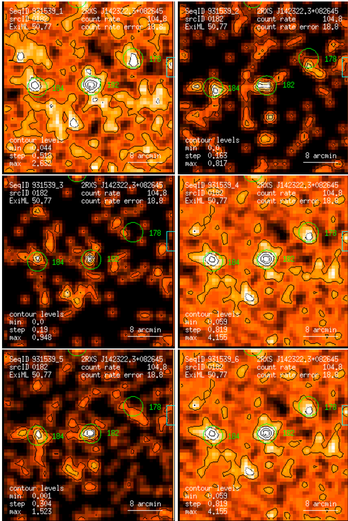
Figure 182: RASS 931539: detection 0182: band rate images, Gaussian filter: (1) PSPC channels 11 – 41, (2) 52 – 90, (3) 91 – 201, (4) 11 – 235, (5) 52 – 201, (6) 11 – 201. Broad band rates in counts/ks. Band rate contour levels in counts/ks/arcmin 2 .
