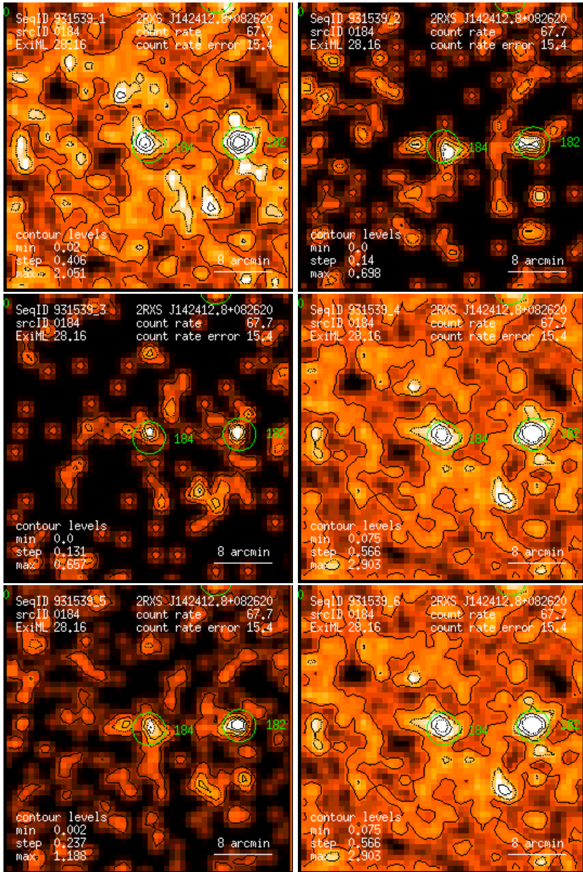
Figure 184: RASS 931539: detection 0184: band rate images, Gaussian filter: (1) PSPC channels 11 – 41, (2) 52 – 90, (3) 91 – 201, (4) 11 – 235, (5) 52 – 201, (6) 11 – 201. Broad band rates in counts/ks. Band rate contour levels in counts/ks/arcmin 2 .
