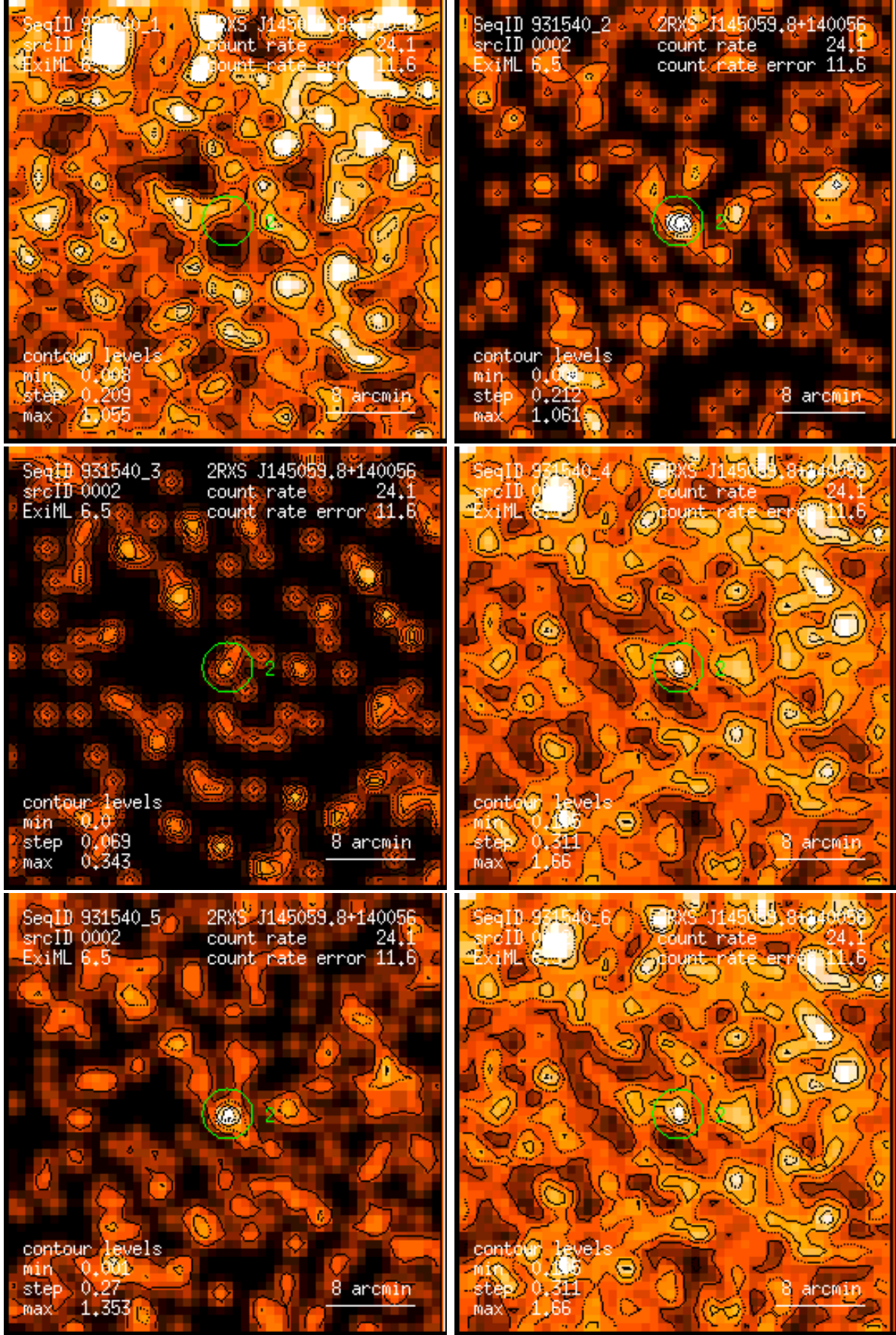
Figure 2: RASS 931540: detection 0002: band rate images, Gaussian filter: (1) PSPC channels 11 – 41, (2) 52 – 90, (3) 91 – 201, (4) 11 – 235, (5) 52 – 201, (6) 11 – 201. Broad band rates in counts/ks. Band rate contour levels in counts/ks/arcmin 2 .
