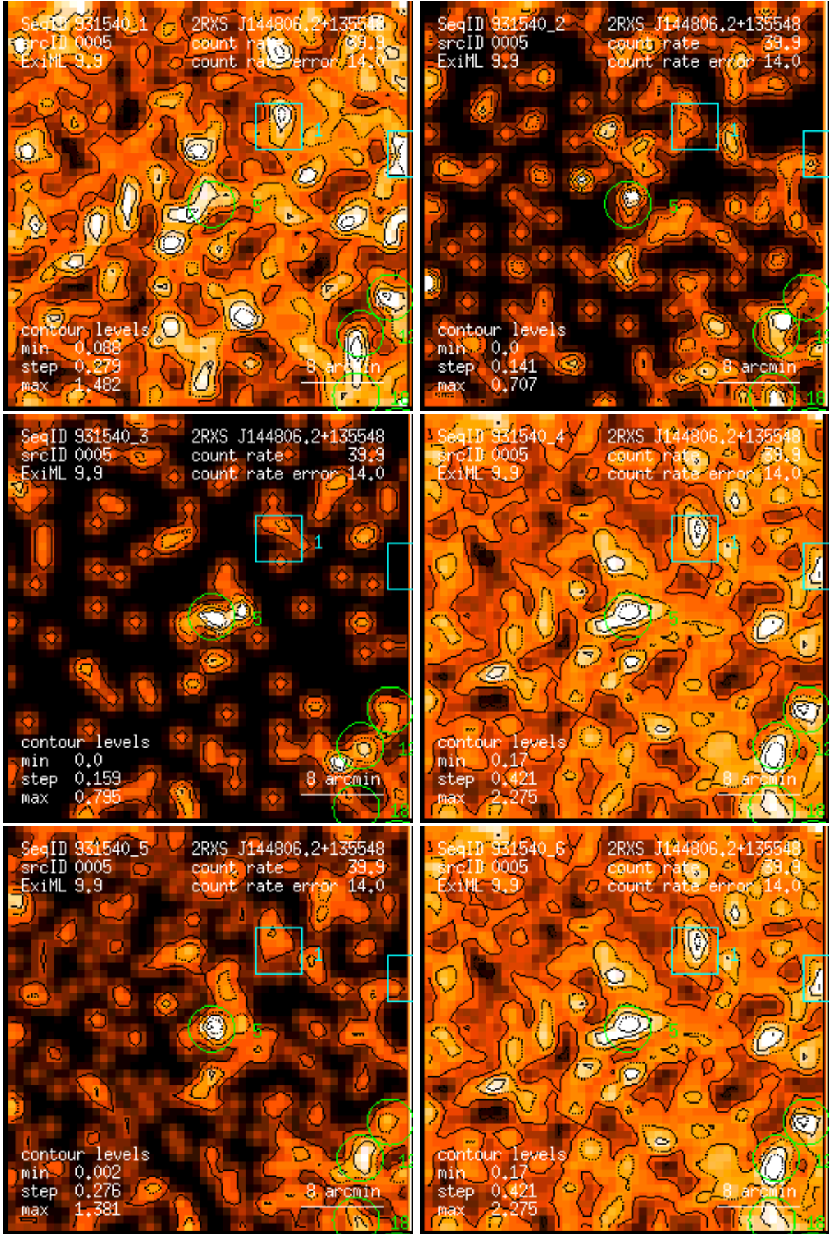
Figure 5: RASS 931540: detection 0005: band rate images, Gaussian filter: (1) PSPC channels 11 – 41, (2) 52 – 90, (3) 91 – 201, (4) 11 – 235, (5) 52 – 201, (6) 11 – 201. Broad band rates in counts/ks. Band rate contour levels in counts/ks/arcmin 2 .
