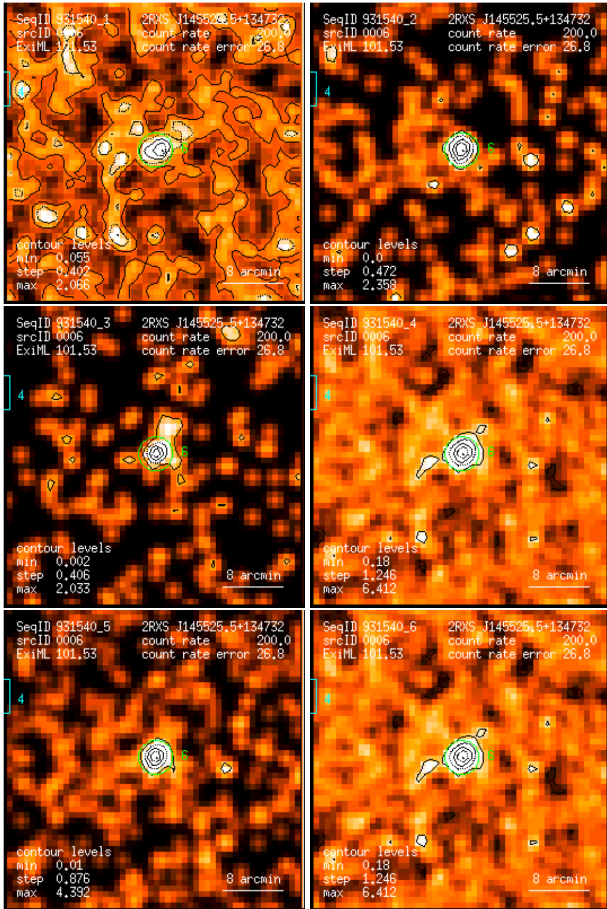
Figure 6: RASS 931540: detection 0006: band rate images, Gaussian filter: (1) PSPC channels 11 – 41, (2) 52 – 90, (3) 91 – 201, (4) 11 – 235, (5) 52 – 201, (6) 11 – 201. Broad band rates in counts/ks. Band rate contour levels in counts/ks/arcmin 2 .
