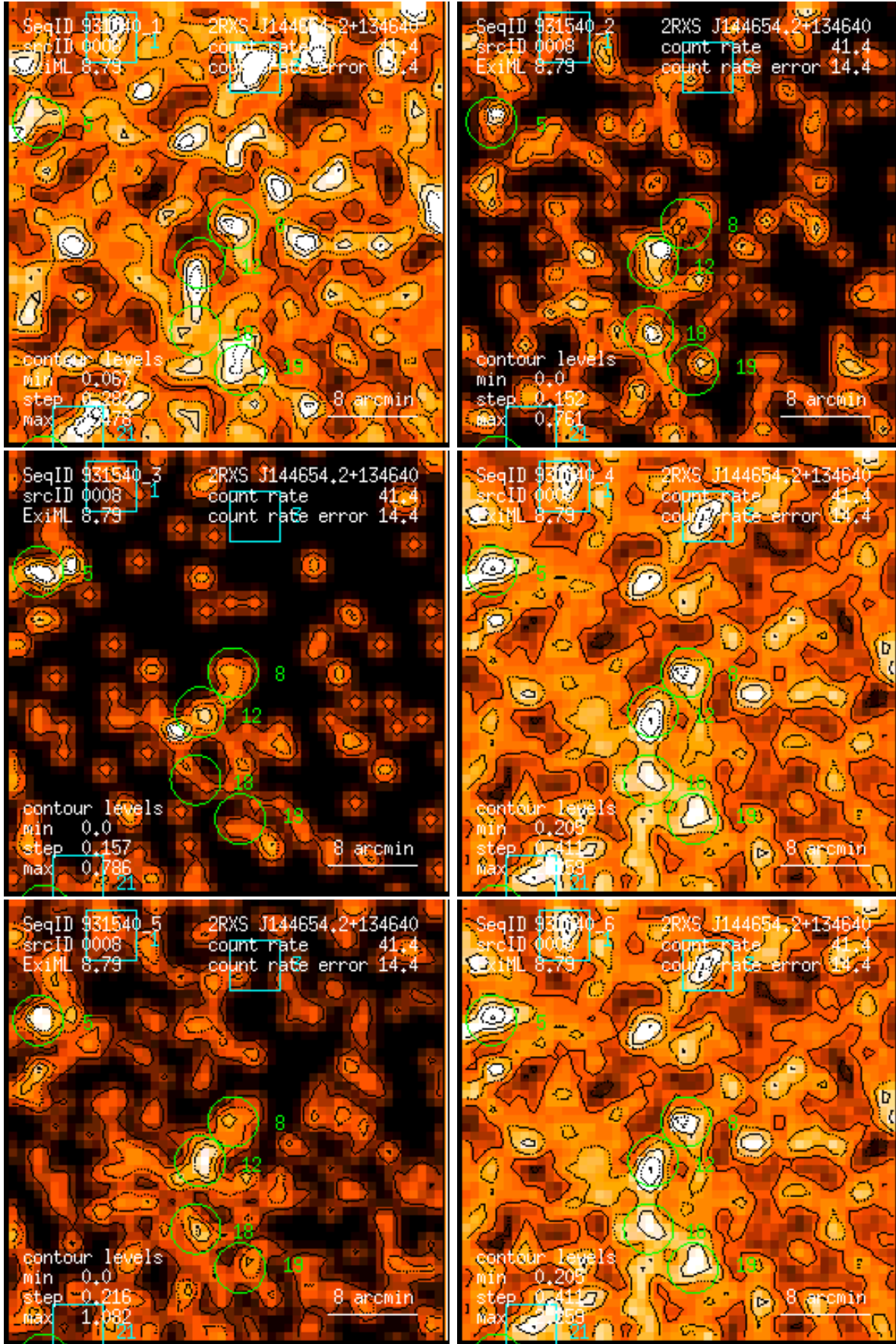
Figure 8: RASS 931540: detection 0008: band rate images, Gaussian filter: (1) PSPC channels 11 – 41, (2) 52 – 90, (3) 91 – 201, (4) 11 – 235, (5) 52 – 201, (6) 11 – 201. Broad band rates in counts/ks. Band rate contour levels in counts/ks/arcmin 2 .
