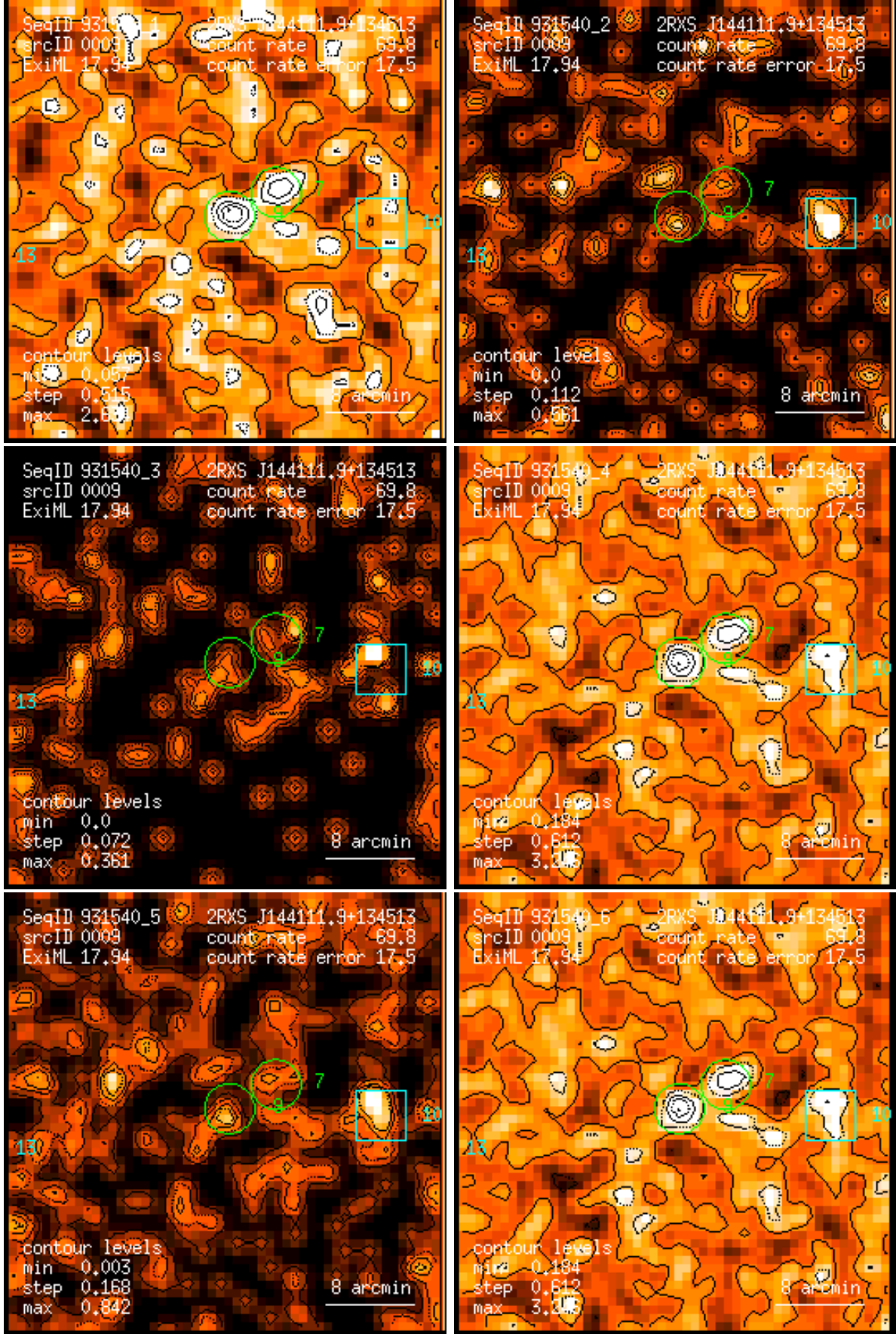
Figure 9: RASS 931540: detection 0009: band rate images, Gaussian filter: (1) PSPC channels 11 – 41, (2) 52 – 90, (3) 91 – 201, (4) 11 – 235, (5) 52 – 201, (6) 11 – 201. Broad band rates in counts/ks. Band rate contour levels in counts/ks/arcmin 2 .
