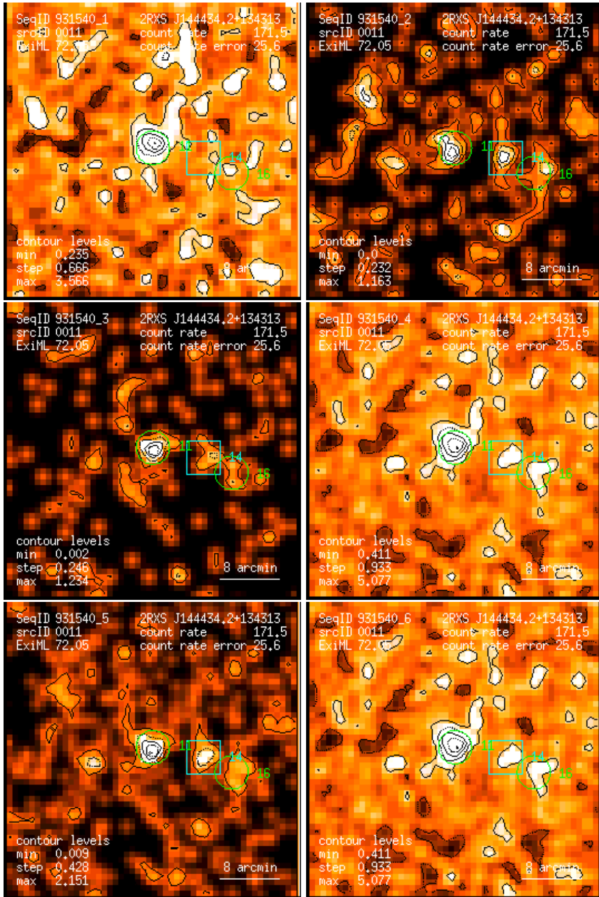
Figure 11: RASS 931540: detection 0011: band rate images, Gaussian filter: (1) PSPC channels 11 – 41, (2) 52 – 90, (3) 91 – 201, (4) 11 – 235, (5) 52 – 201, (6) 11 – 201. Broad band rates in counts/ks. Band rate contour levels in counts/ks/arcmin 2 .
