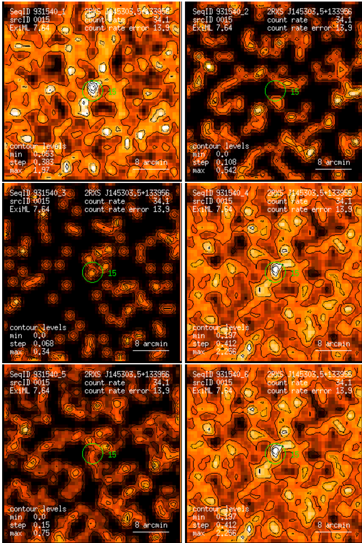
Figure 15: RASS 931540: detection 0015: band rate images, Gaussian filter: (1) PSPC channels 11 – 41, (2) 52 – 90, (3) 91 – 201, (4) 11 – 235, (5) 52 – 201, (6) 11 – 201. Broad band rates in counts/ks. Band rate contour levels in counts/ks/arcmin 2 .
