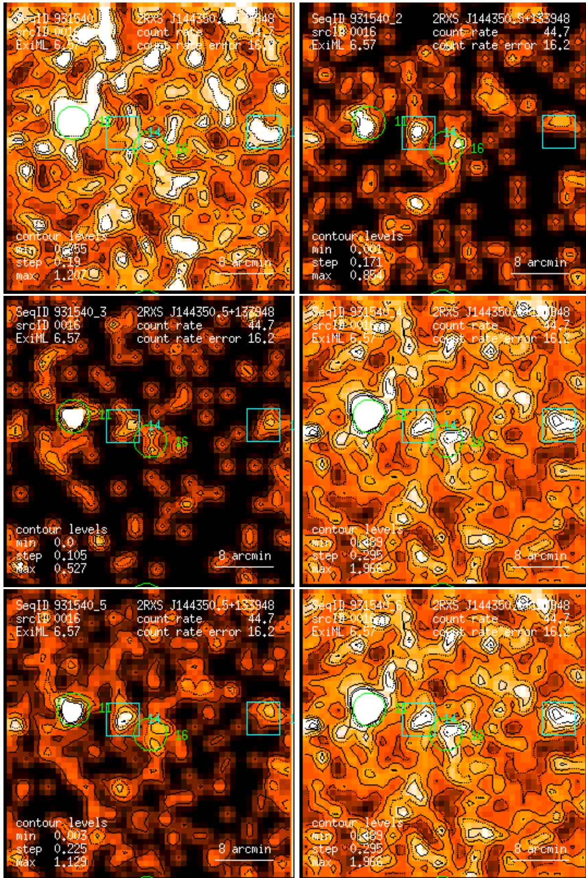
Figure 16: RASS 931540: detection 0016: band rate images, Gaussian filter: (1) PSPC channels 11 – 41, (2) 52 – 90, (3) 91 – 201, (4) 11 – 235, (5) 52 – 201, (6) 11 – 201. Broad band rates in counts/ks. Band rate contour levels in counts/ks/arcmin 2 .
