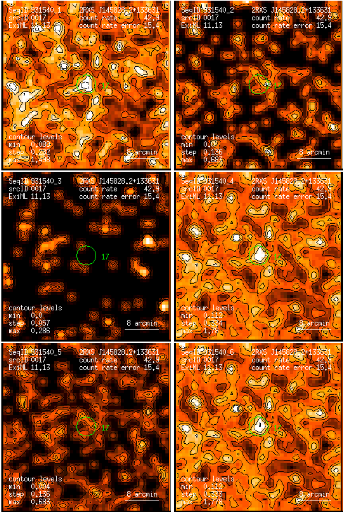
Figure 17: RASS 931540: detection 0017: band rate images, Gaussian filter: (1) PSPC channels 11 – 41, (2) 52 – 90, (3) 91 – 201, (4) 11 – 235, (5) 52 – 201, (6) 11 – 201. Broad band rates in counts/ks. Band rate contour levels in counts/ks/arcmin 2 .
