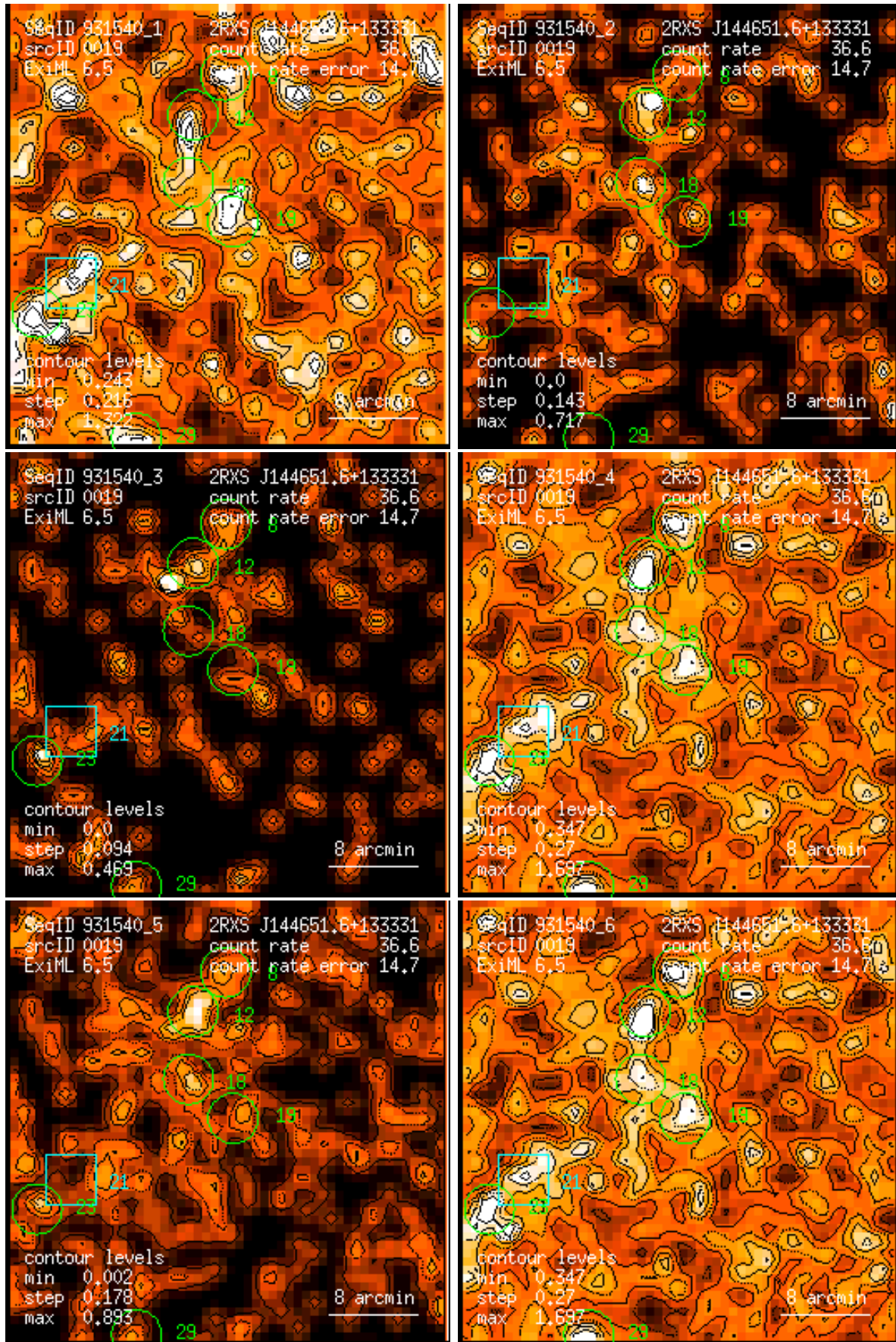
Figure 19: RASS 931540: detection 0019: band rate images, Gaussian filter: (1) PSPC channels 11 – 41, (2) 52 – 90, (3) 91 – 201, (4) 11 – 235, (5) 52 – 201, (6) 11 – 201. Broad band rates in counts/ks. Band rate contour levels in counts/ks/arcmin 2 .
