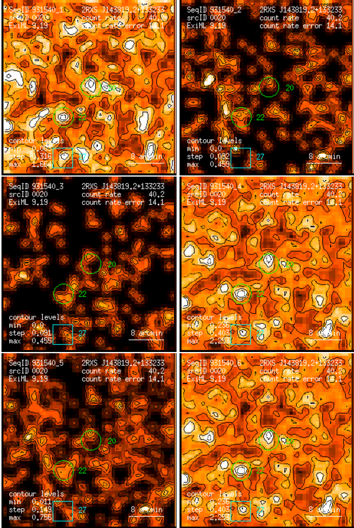
Figure 20: RASS 931540: detection 0020: band rate images, Gaussian filter: (1) PSPC channels 11 – 41, (2) 52 – 90, (3) 91 – 201, (4) 11 – 235, (5) 52 – 201, (6) 11 – 201. Broad band rates in counts/ks. Band rate contour levels in counts/ks/arcmin 2 .
