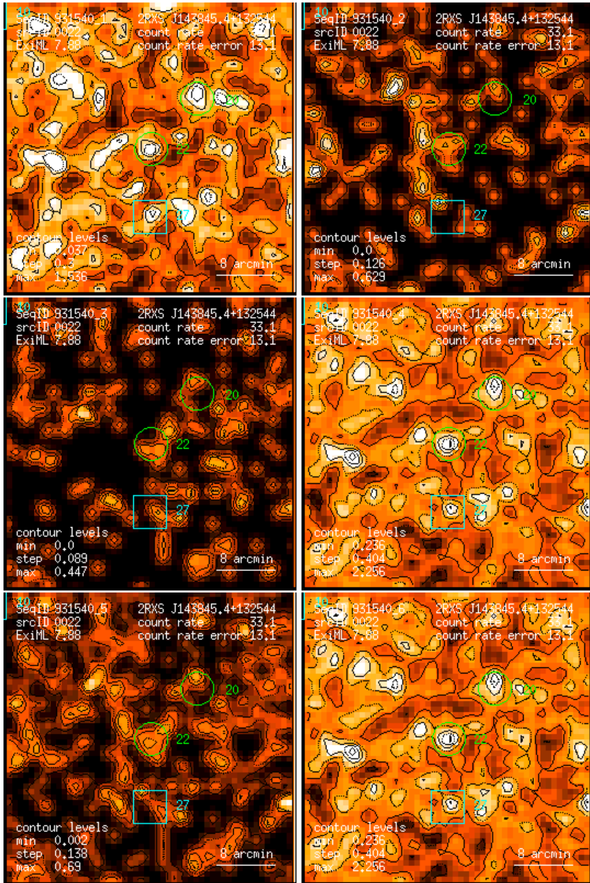
Figure 22: RASS 931540: detection 0022: band rate images, Gaussian filter: (1) PSPC channels 11 – 41, (2) 52 – 90, (3) 91 – 201, (4) 11 – 235, (5) 52 – 201, (6) 11 – 201. Broad band rates in counts/ks. Band rate contour levels in counts/ks/arcmin 2 .
