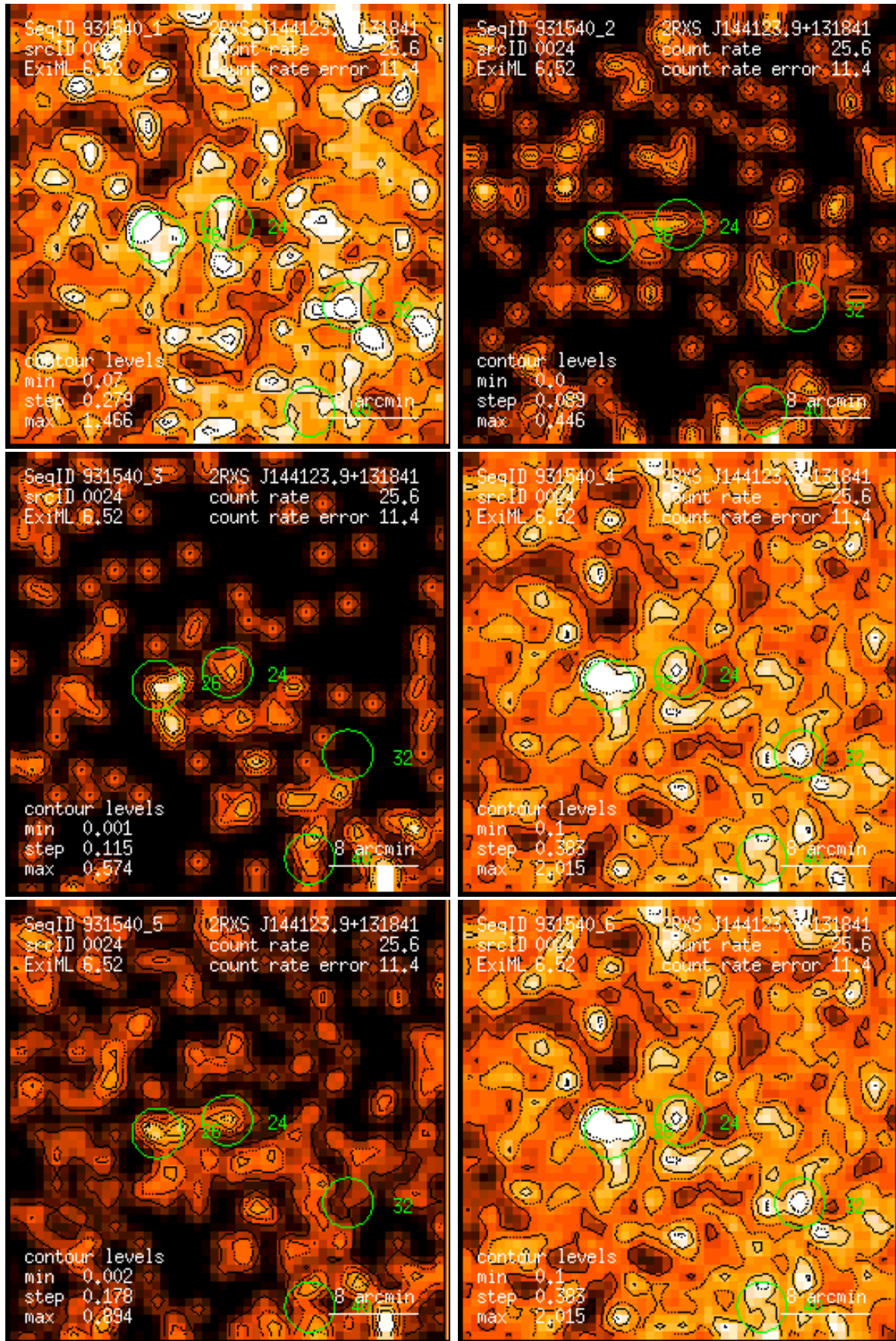
Figure 24: RASS 931540: detection 0024: band rate images, Gaussian filter: (1) PSPC channels 11 – 41, (2) 52 – 90, (3) 91 – 201, (4) 11 – 235, (5) 52 – 201, (6) 11 – 201. Broad band rates in counts/ks. Band rate contour levels in counts/ks/arcmin 2 .
