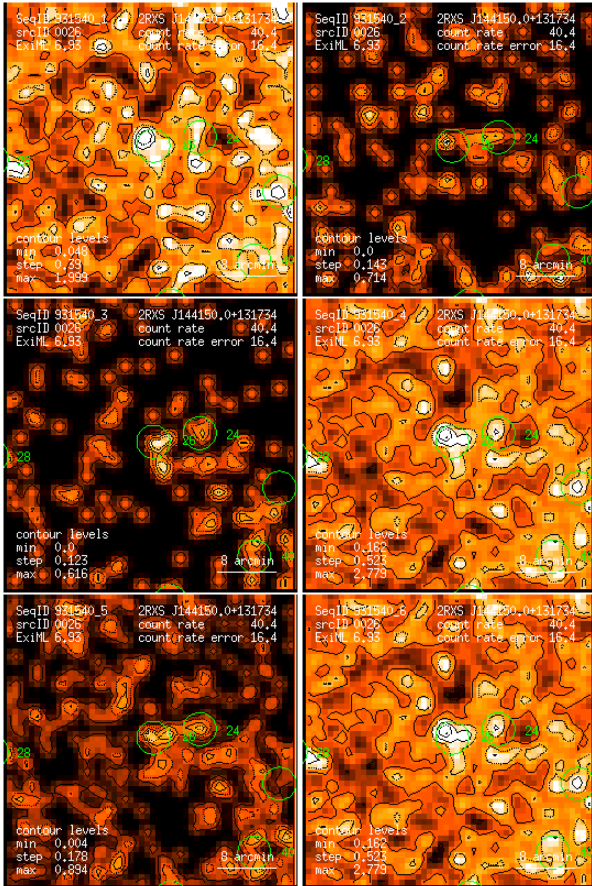
Figure 26: RASS 931540: detection 0026: band rate images, Gaussian filter: (1) PSPC channels 11 – 41, (2) 52 – 90, (3) 91 – 201, (4) 11 – 235, (5) 52 – 201, (6) 11 – 201. Broad band rates in counts/ks. Band rate contour levels in counts/ks/arcmin 2 .
